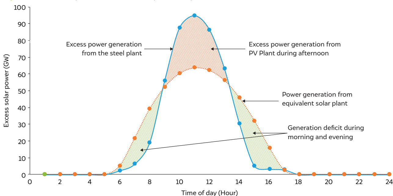
Figure 10 Time-of-day excess solar electricity for Bellary, Karnataka
