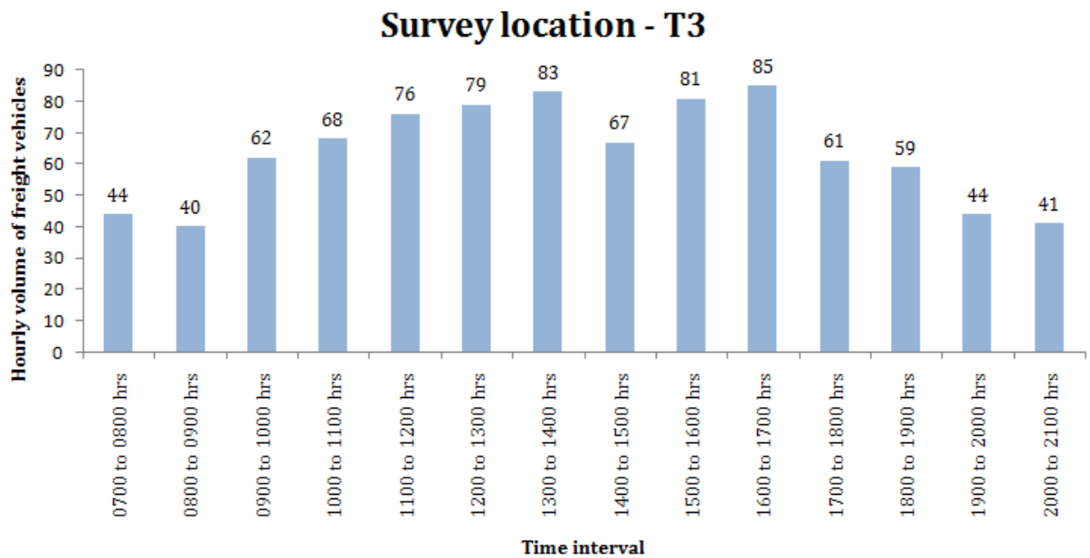
Figure 10: Hourly variation in freight vehicle traffic volume on Sir Theagaraya Road (T3)
