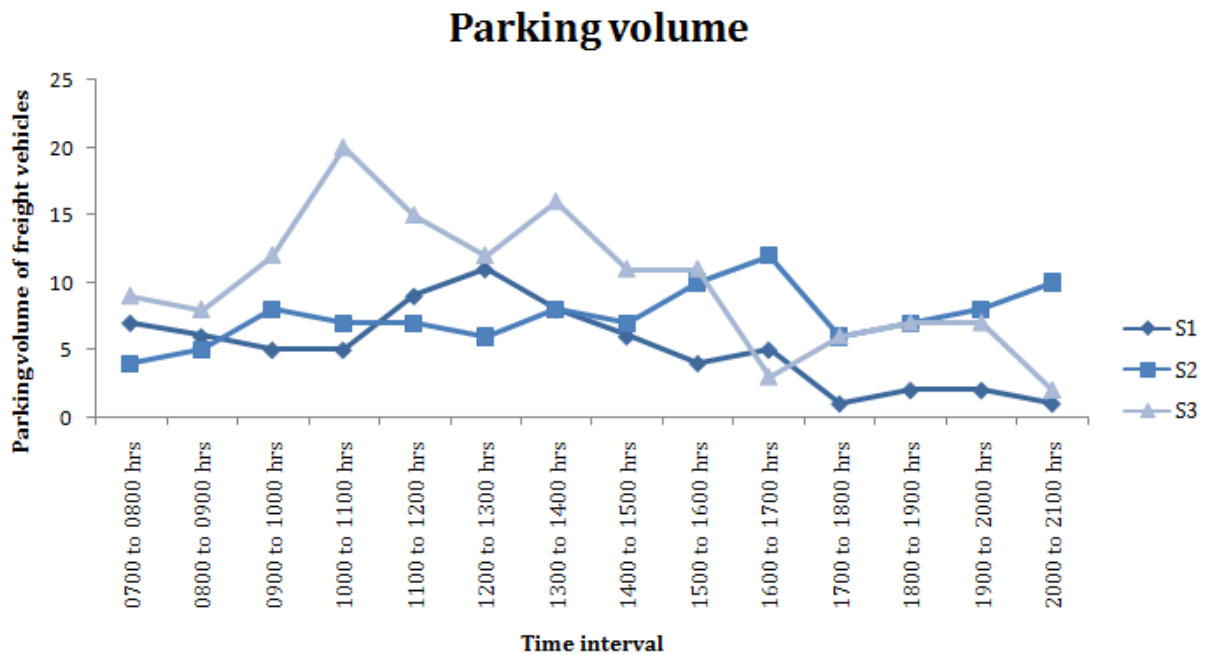
Figure 17: Hourly variation in freight vehicle parking volume
