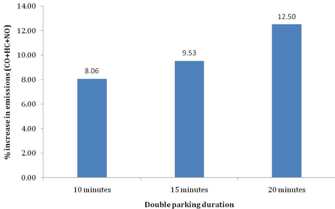
Figure 22: Increase in emissions due to double parking compared to dedicated parking
