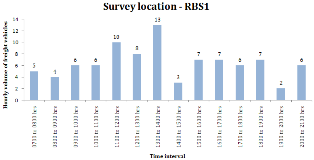
Figure 11: Hourly variation in freight vehicle traffic volume on Raja Bather Street (RBS1)
