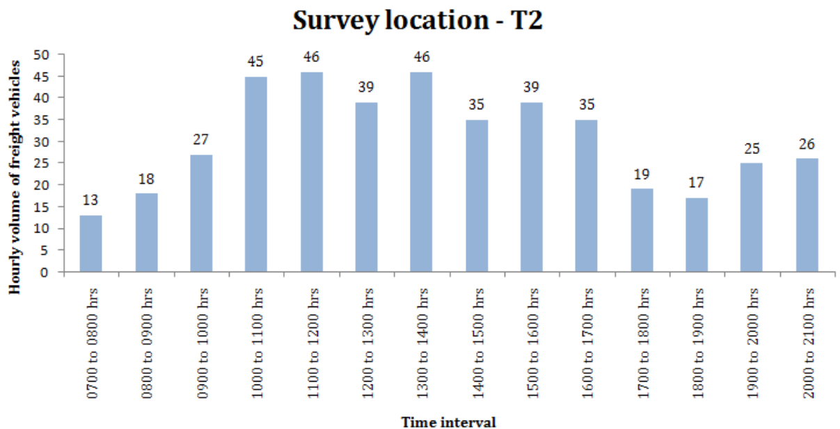
Figure 9: Hourly variation in freight vehicle traffic volume on Sir Theagaraya Road (T2)
