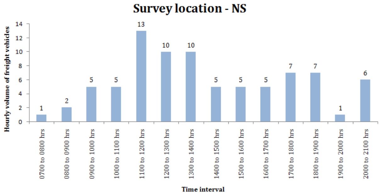
Figure 13: Hourly variation in freight vehicle traffic volume on Nana Street
