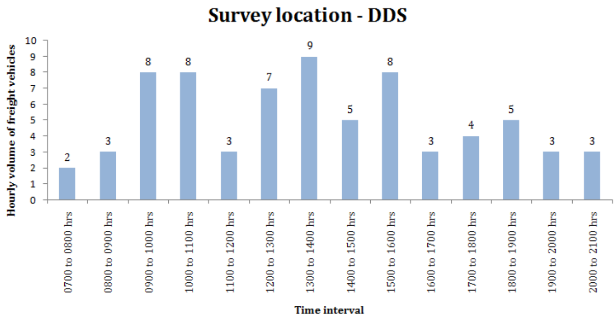
Figure 14: Hourly variation in freight vehicle traffic volume on Deena Dayalu Street
