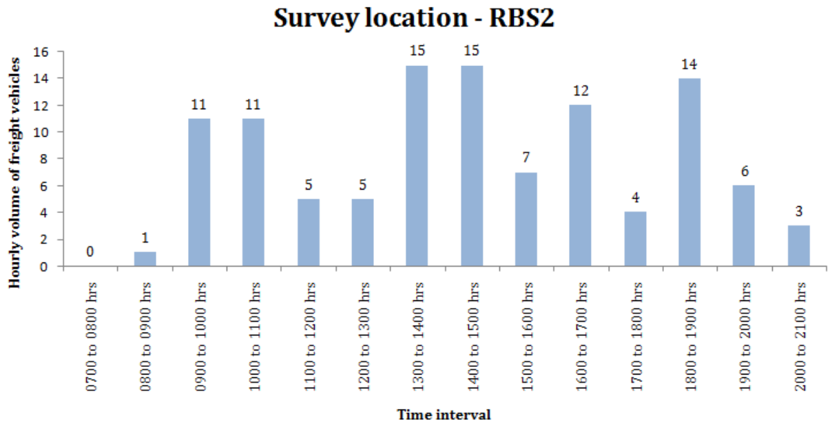
Figure 12: Hourly variation in freight vehicle traffic volume on Raja Bather Street (RBS2)
