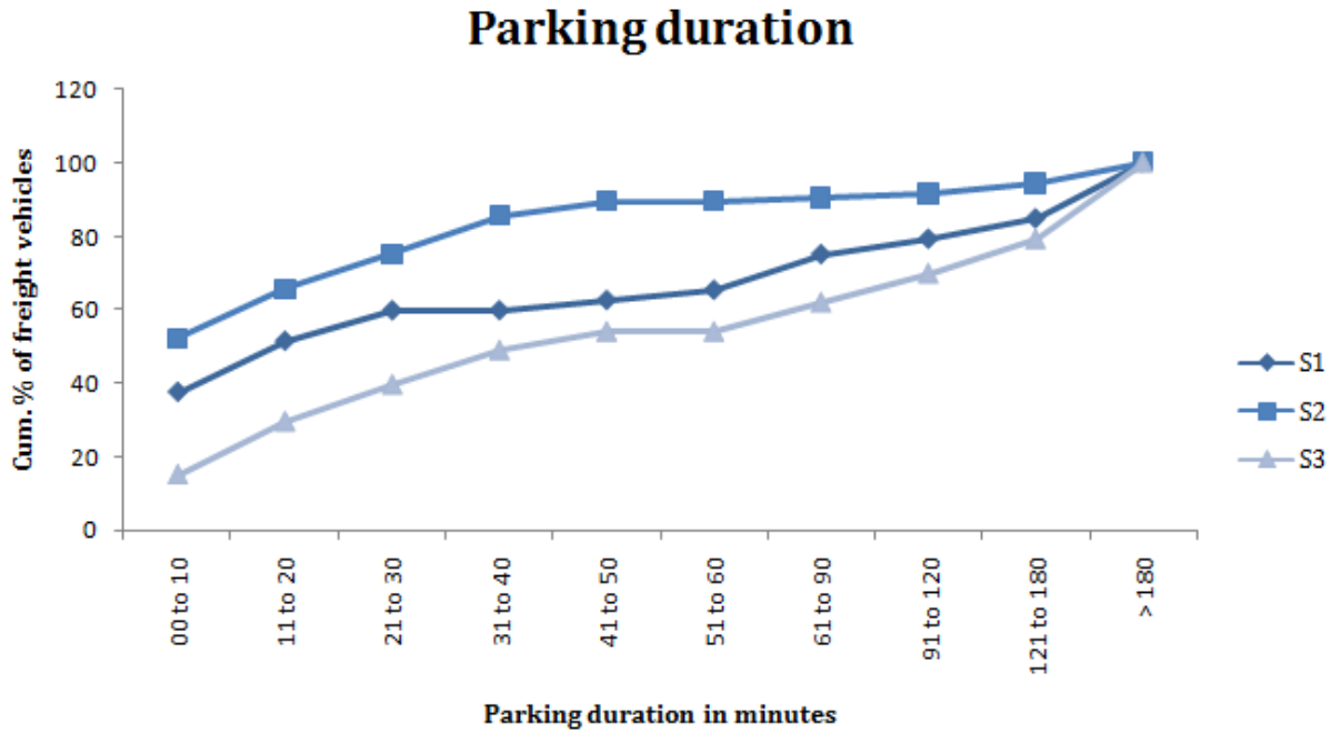
Figure 18: Freight vehicle parking duration
