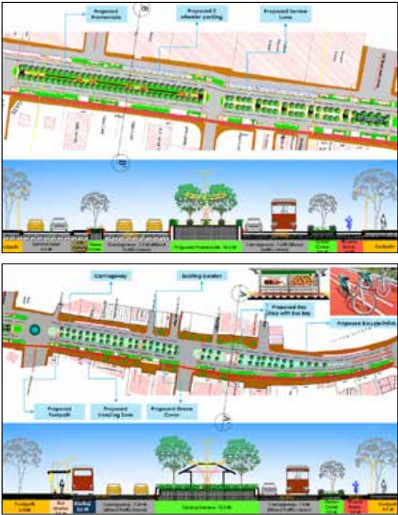
Figure 16: Excerpts of Design Proposal for Hiran Magri Smart Road
