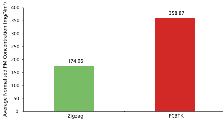
Figure 3: Overall average corrected PM concentrations in zigzag brick kilns and FCBTKs
