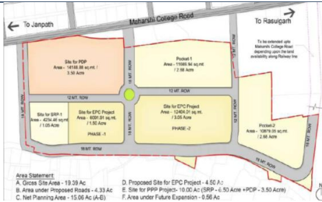
Figure 21: Site Layout – Odisha
