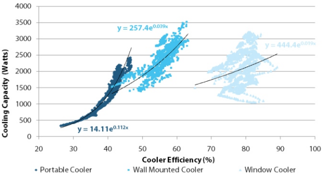
Fig3 Comparison of Cooling Capacity and Cooling Efficiency of different coolers
