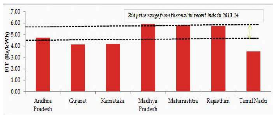
Figure 2: Thermal bids Vs Wind FIT in 2013-14
