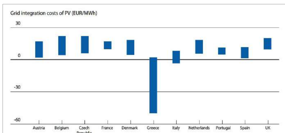
Figure 6: Integration Costs for Solar PV in The European Union for Between 2% and 18% of Electricity Generation with Demand Response (Source: Pudjianto 2013)
