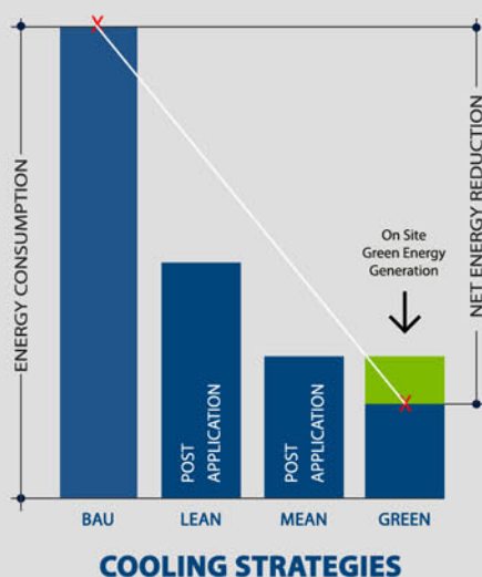
Potential energy savings from a sequential Lean-Mean-Green approach
