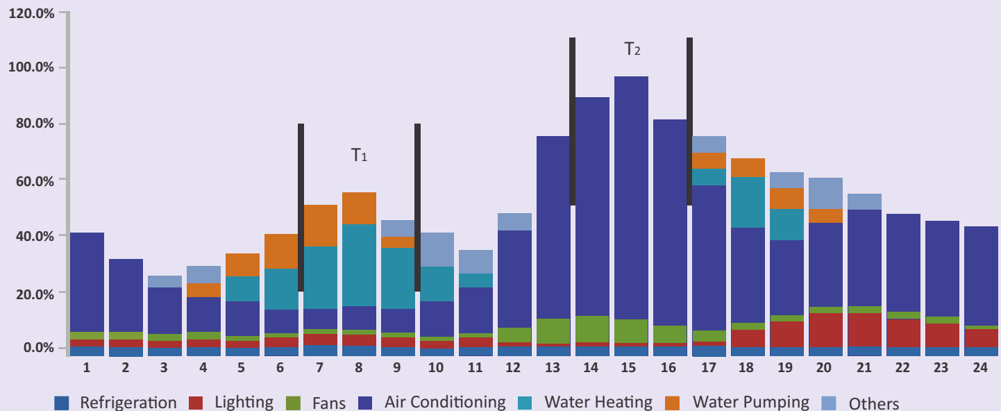
Figure 2: Typical Residential Load Curve (e.g. during summer in Delhi)
