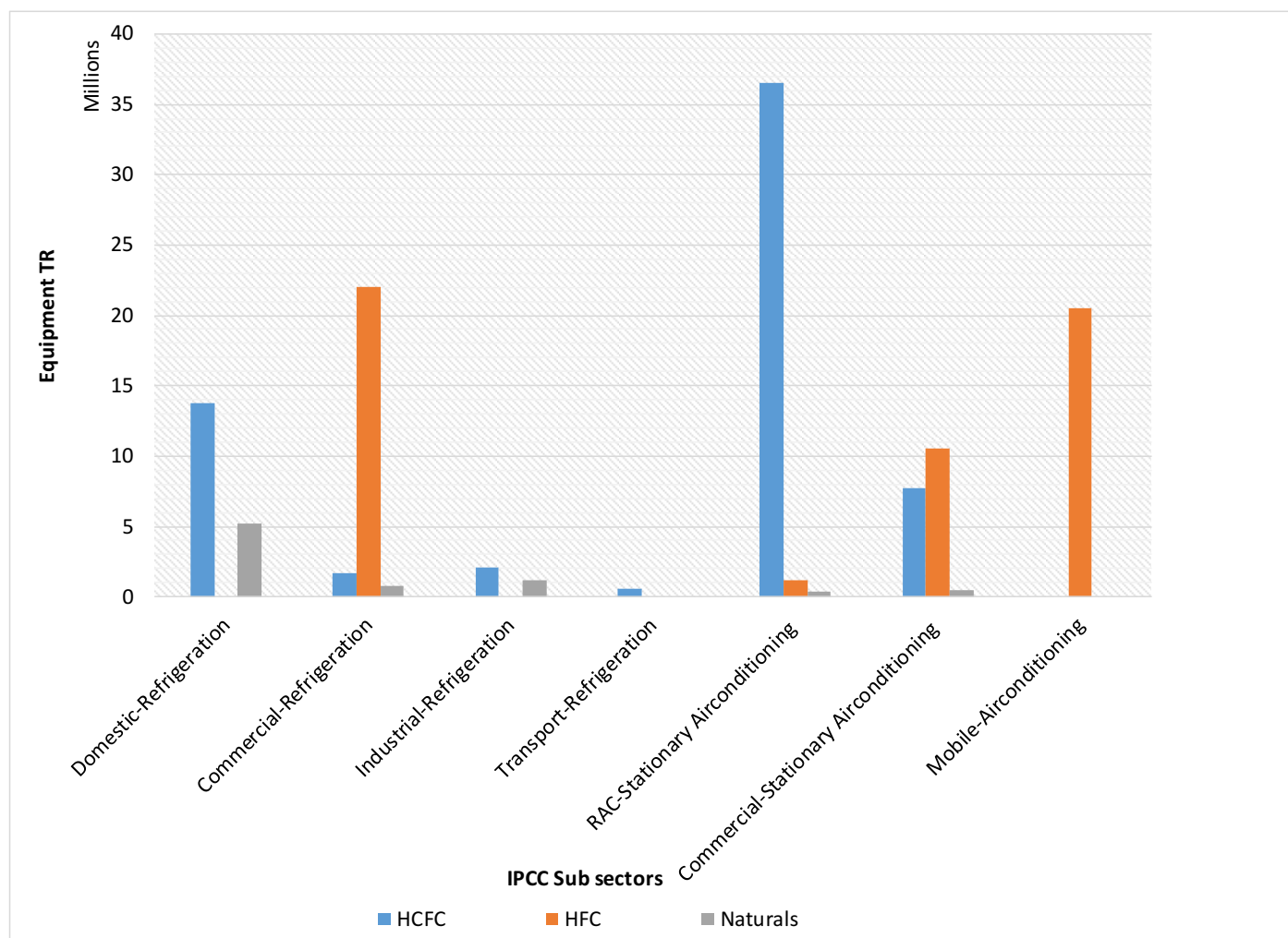
Figure 7 | IPCC Sector wise Refrigerant Equipment TR (2015)
