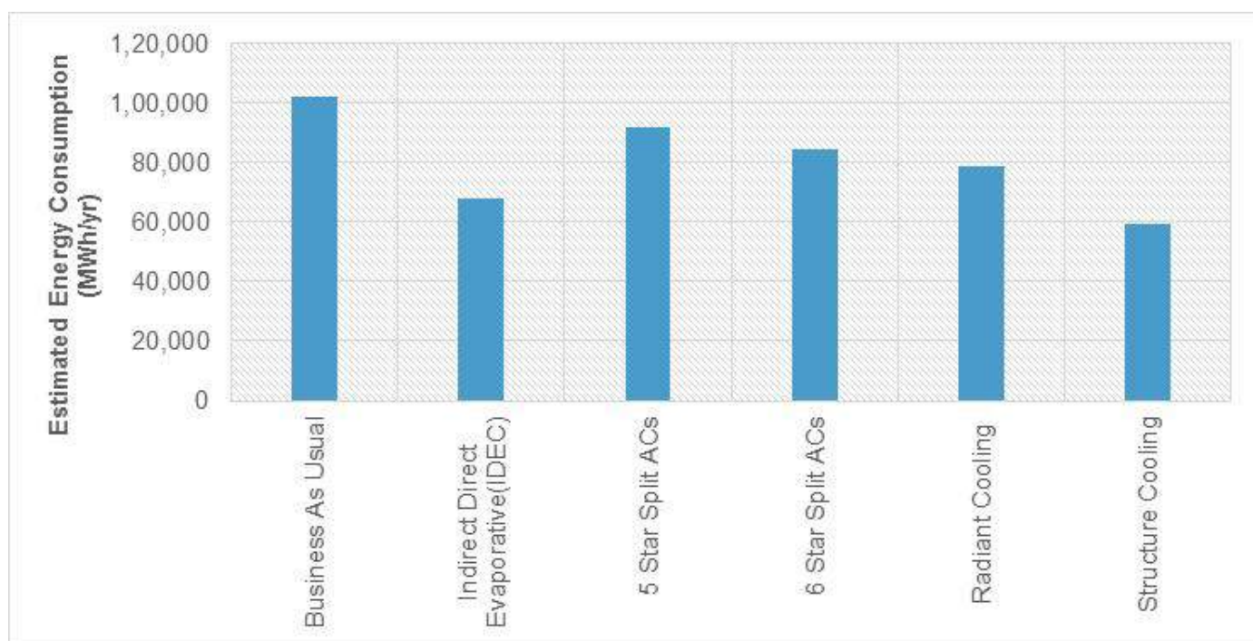
Figure 58 | Energy Consumption - Conventional & Natural Refrigerant based technologies
