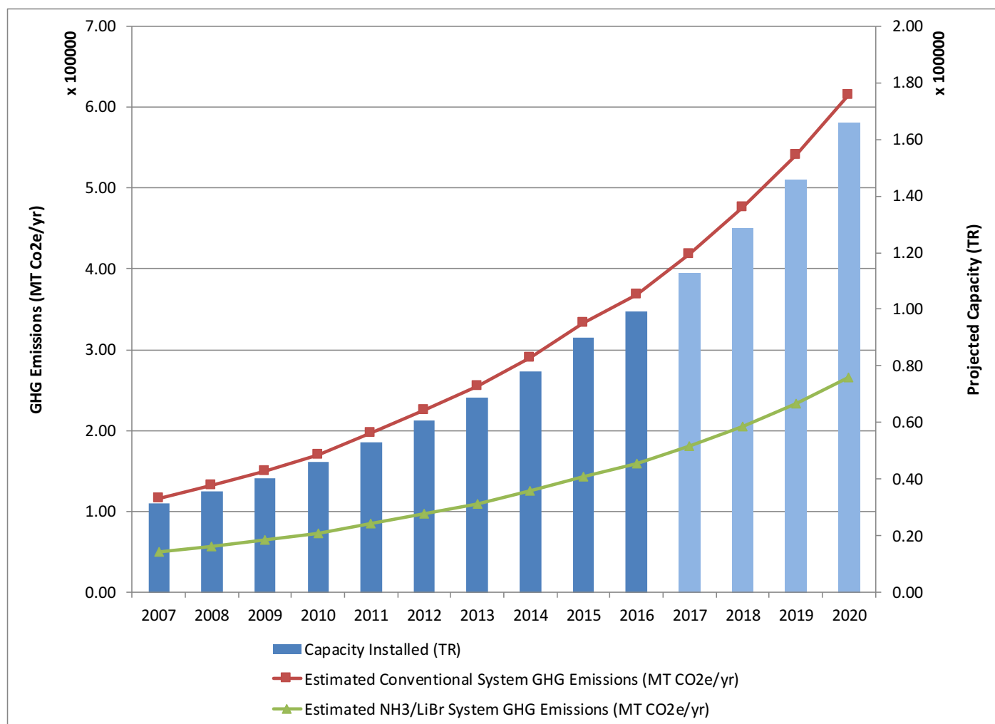
Figure 35 | NH3/LiBr VAM Growth (TR) & GHG Emission Projection (BAU Scenario)
