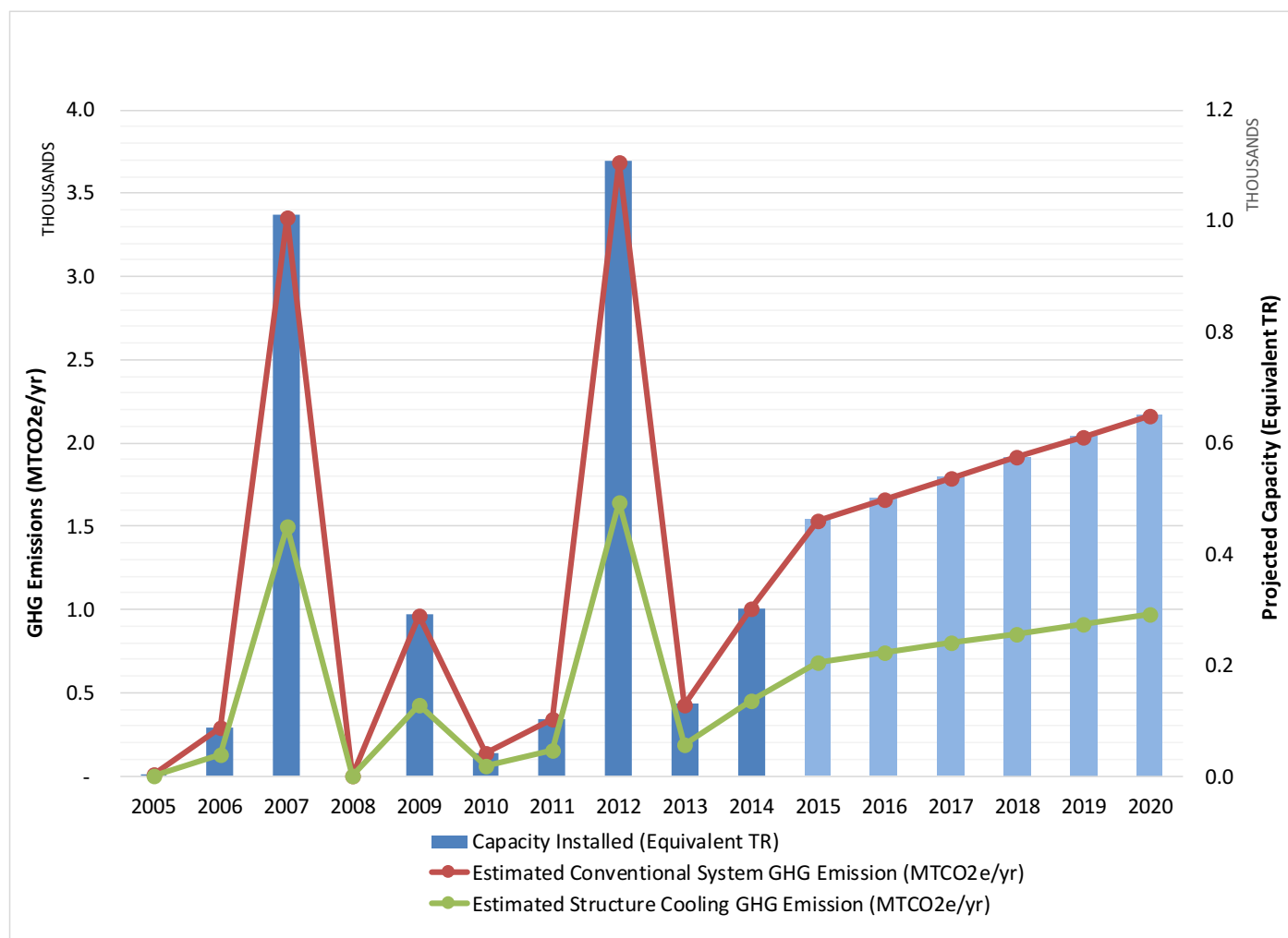
Figure 43 | Structure Cooling Growth (TR) & GHG Emission Projection
