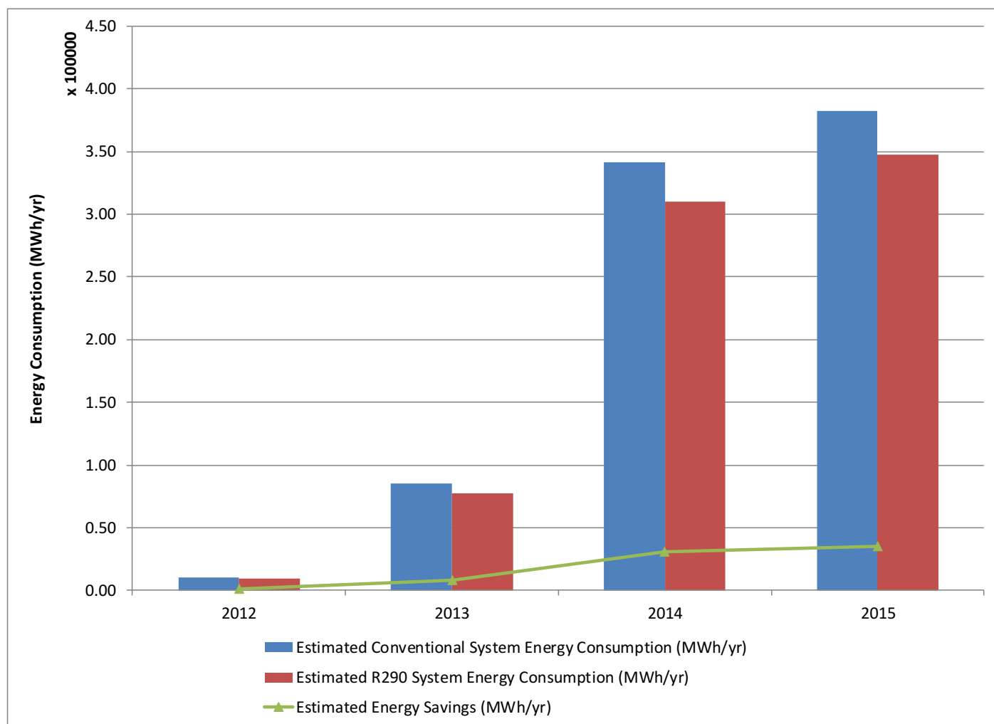
Figure 21 | Energy Consumption: Conventional System vs R290 System
