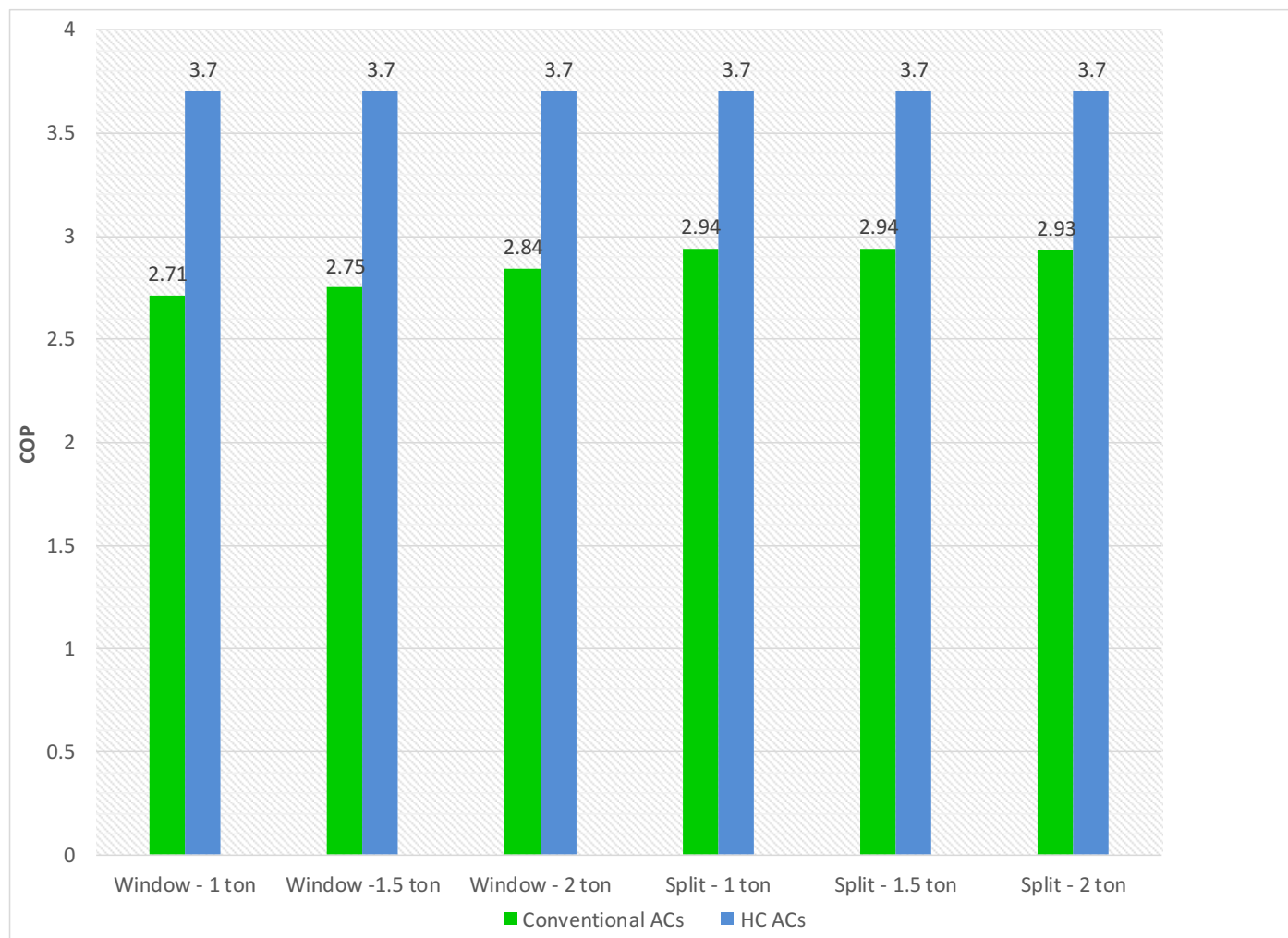
Figure 27 | COP comparison of conventional ACs vs HC ACs
