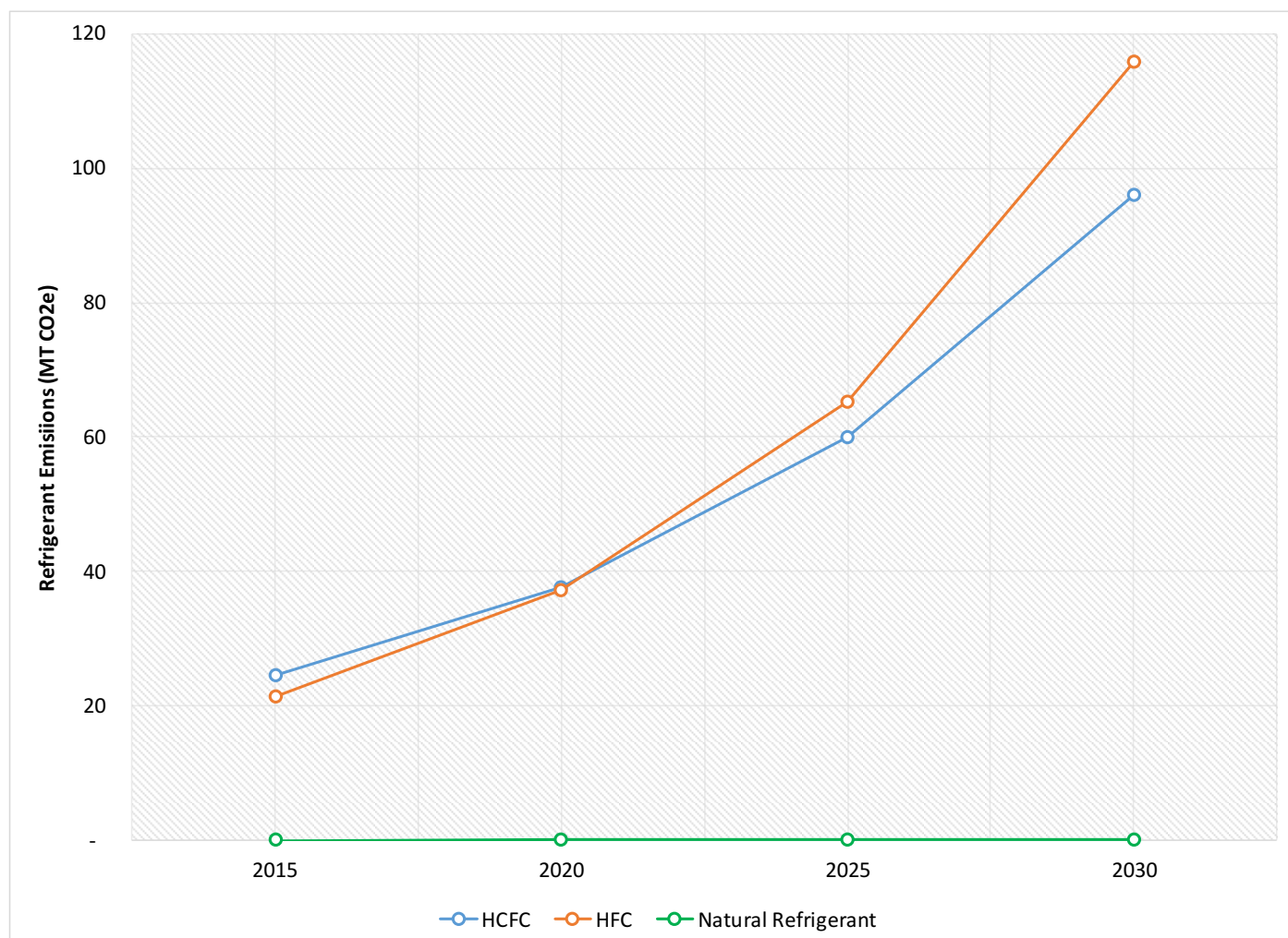
Figure 12 | Refrigerant Emissions Projection (2015-2030)
