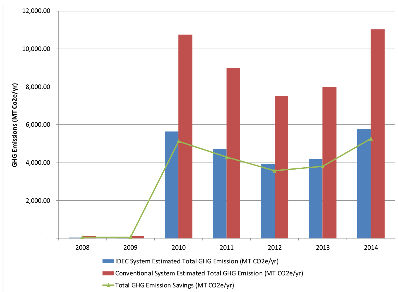
Figure 50 | GHG Emissions: Conventional System vs IDEC System
