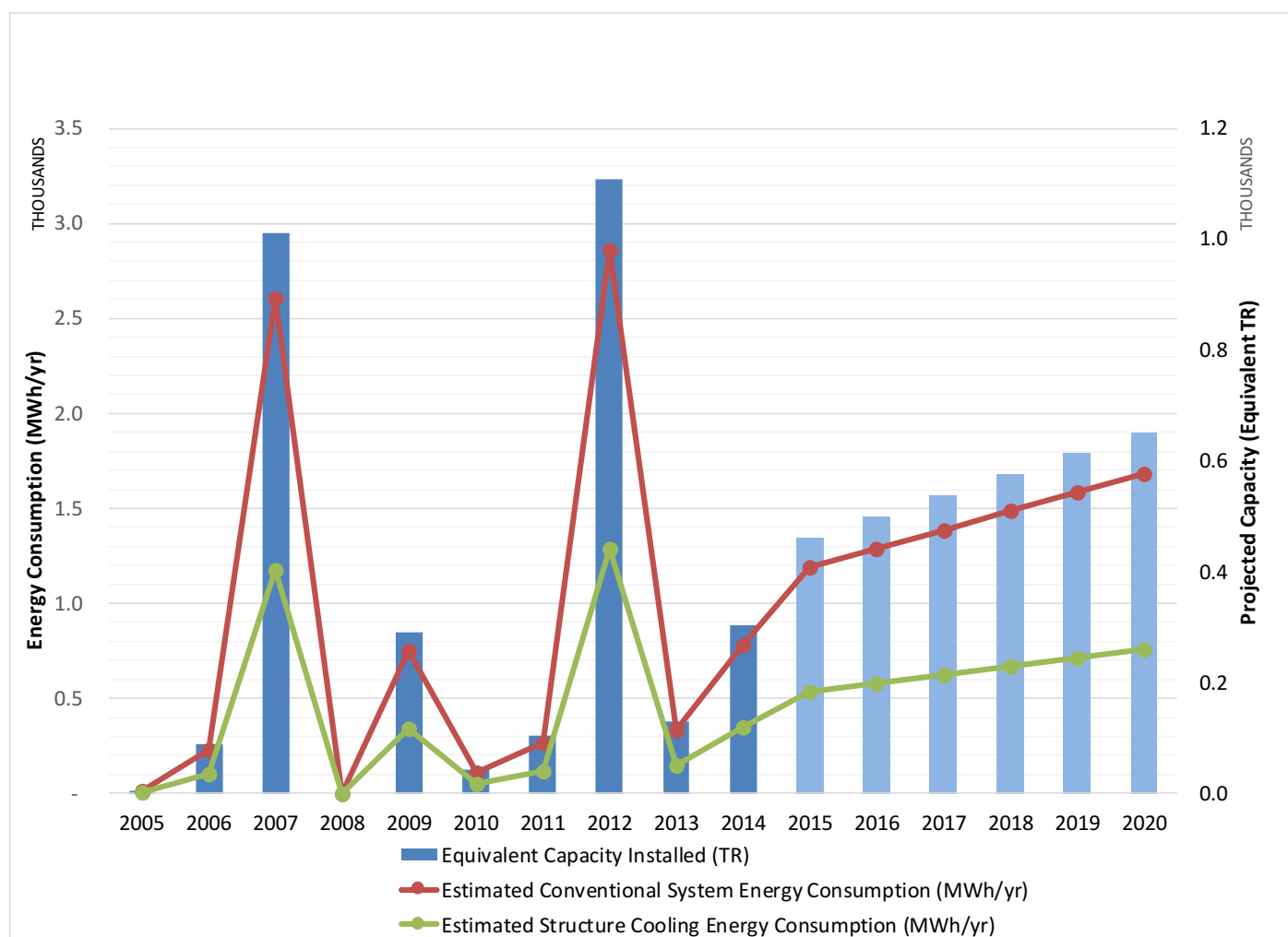
Figure 42 | Structure Cooling Growth (TR) & Energy Consumption Projection
