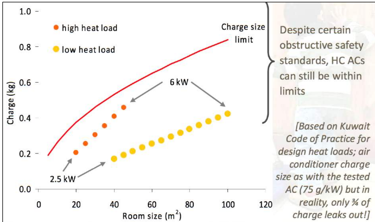
Figure 31 | Charge size limit of R290
