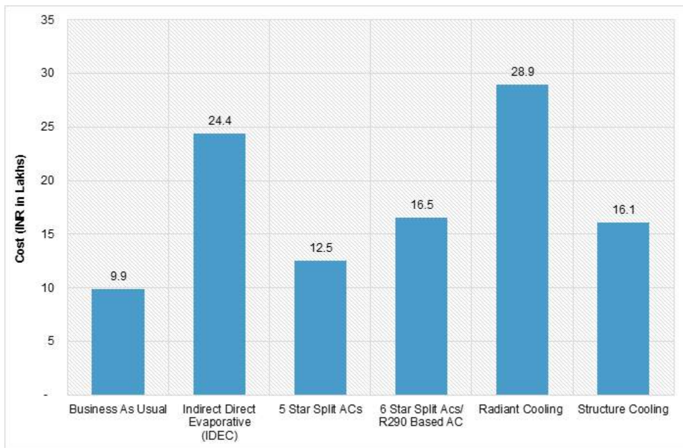
Figure 60 | Capital Costs - Conventional & Natural Refrigerant based technologies
