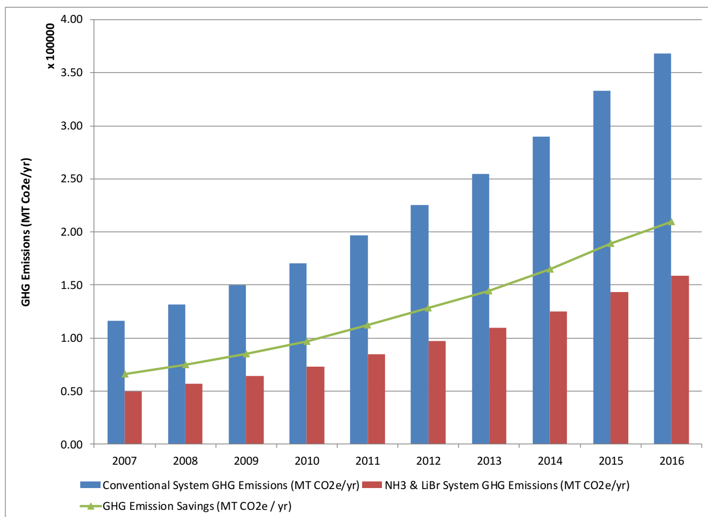
Figure 33 | GHG Emission: Conventional System vs NH 3 /LiBr System
