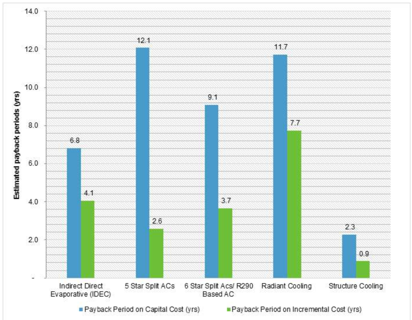
Figure 61 | Payback Period - Conventional & Natural Refrigerant based technologies
