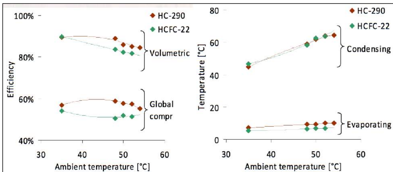
Figure 30 | Comparison of R22 and R290 ACs: III
