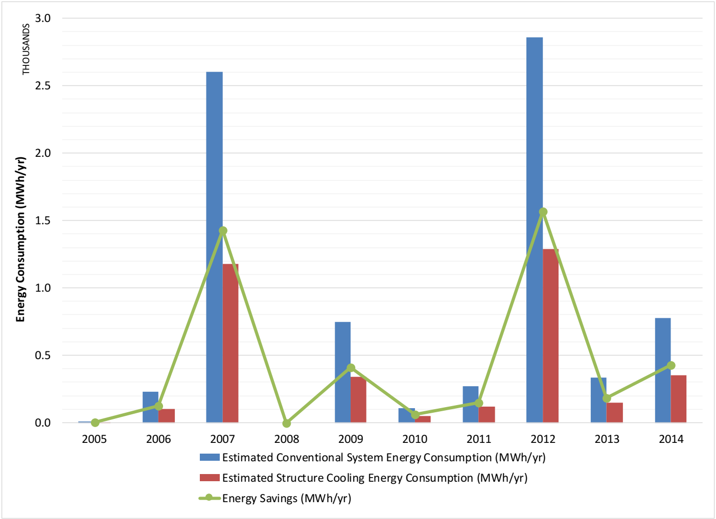
Figure 40 | Energy Consumption: Conventional vs Structure Cooling
