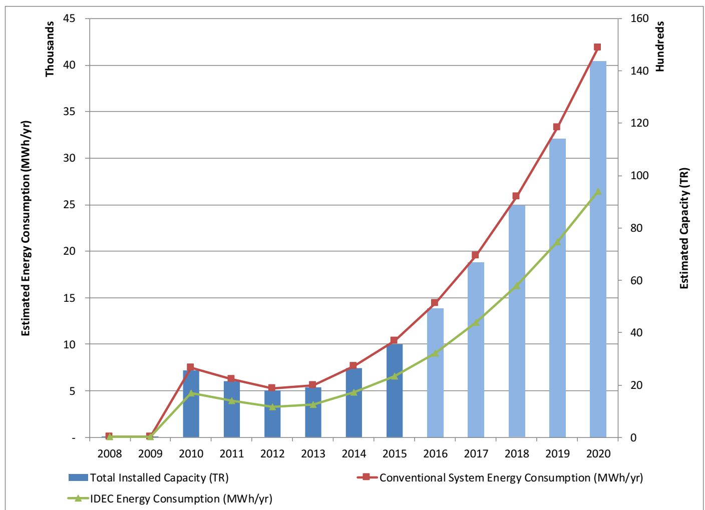
Figure 51 | IDEC System Growth (TR) & Energy Consumption Projection
