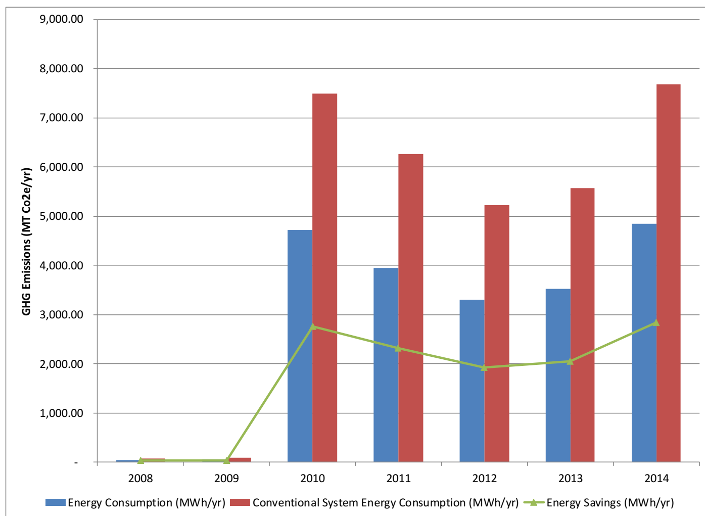
Figure 49 | Energy Consumption: Conventional System vs IDEC System
