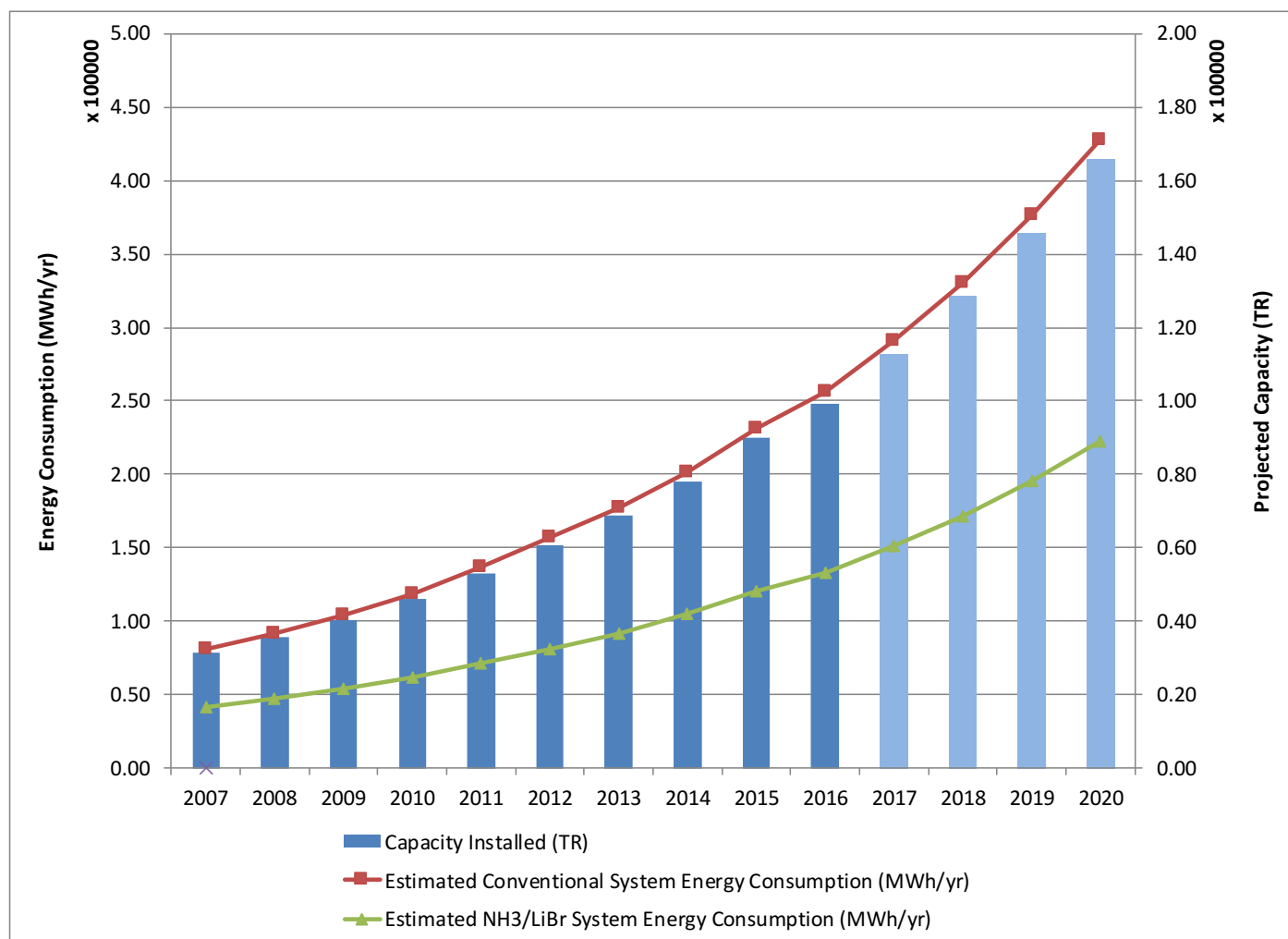
Figure 34 | NH 3 /LiBr VAM Growth (TR) & Energy Consump. Projection (BAU Scenario)
