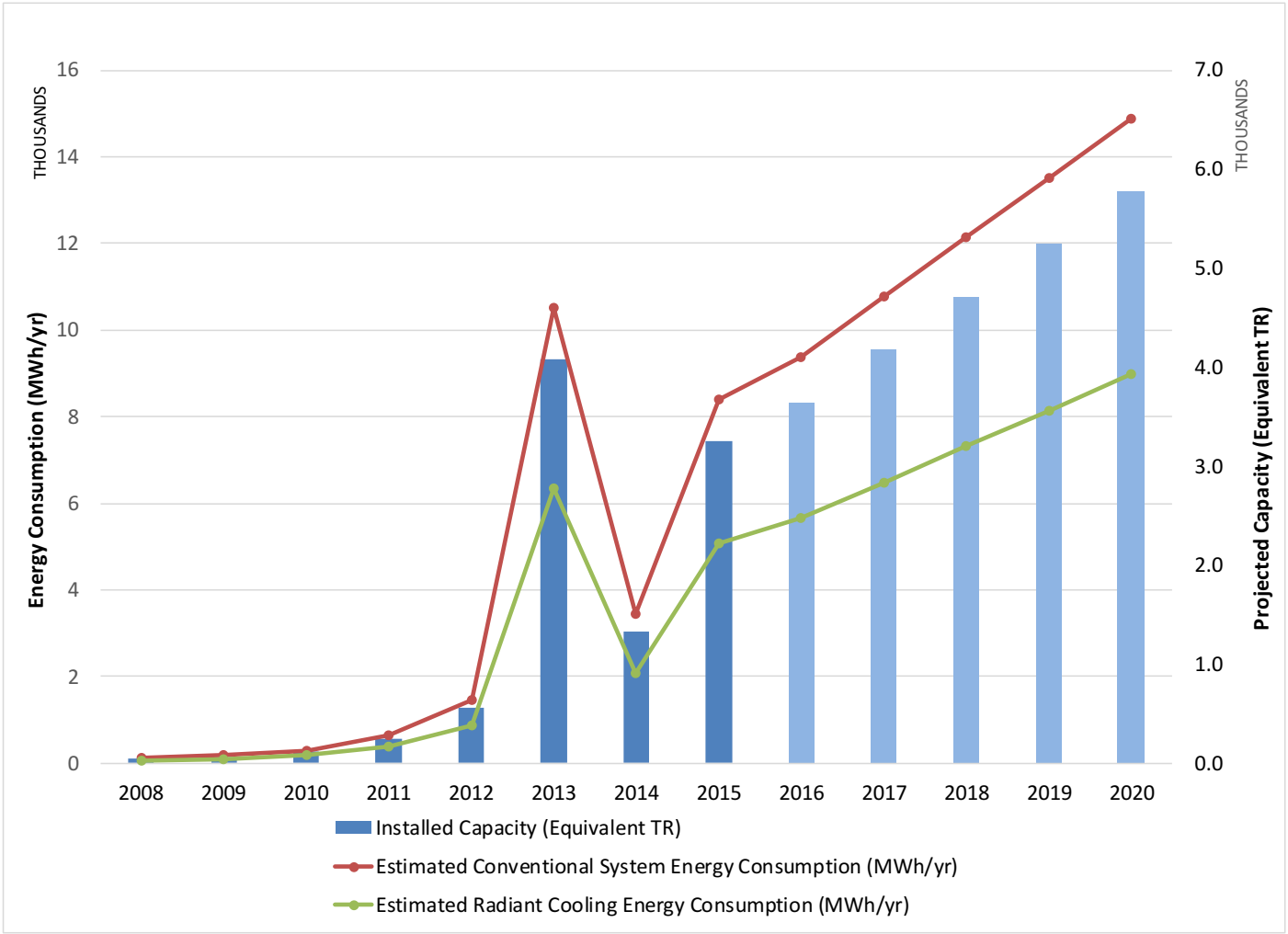
Figure 46 | Radiant Cooling Growth (TR) & Energy Consumption Projection
