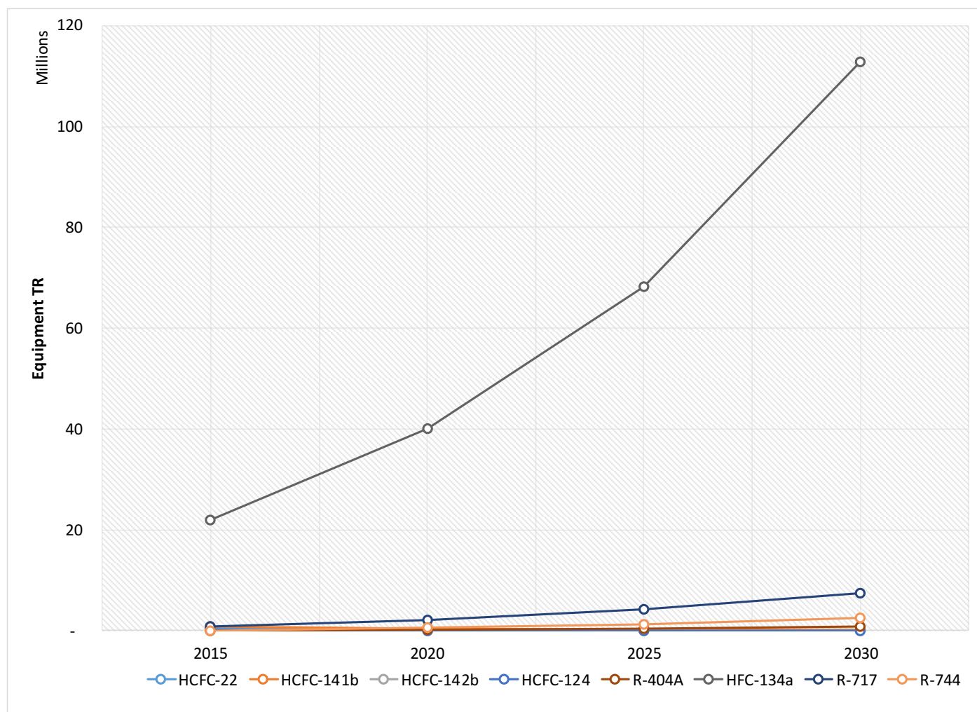
Figure 14 | Commercial Refrigeration Equipment TR Projections (2015-2030)
