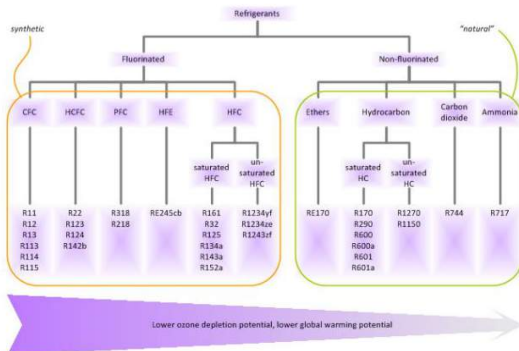
Figure 4 | Classification of Refrigerants
