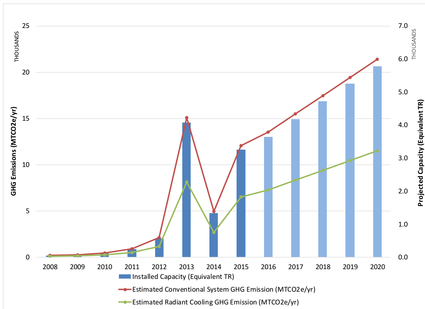
Figure 47 | Radiant Cooling Growth (TR) & GHG Emission Projection
