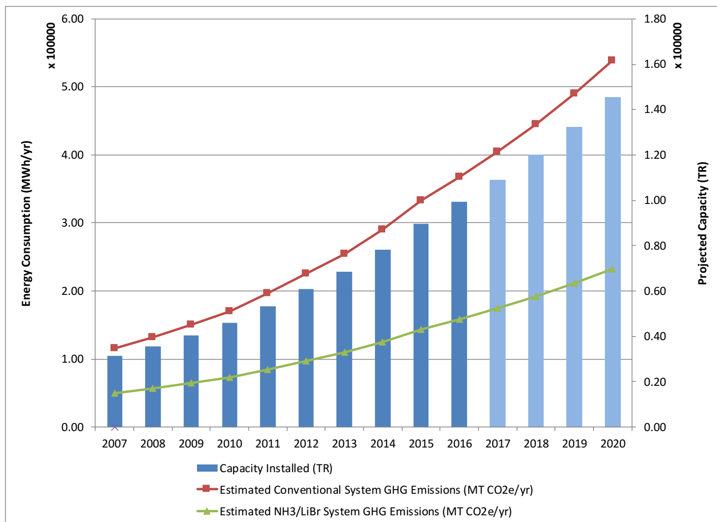
Figure 37 | NH3/LiBr VAM Growth (TR) & GHG Emission Projection (MGR Scenario)
