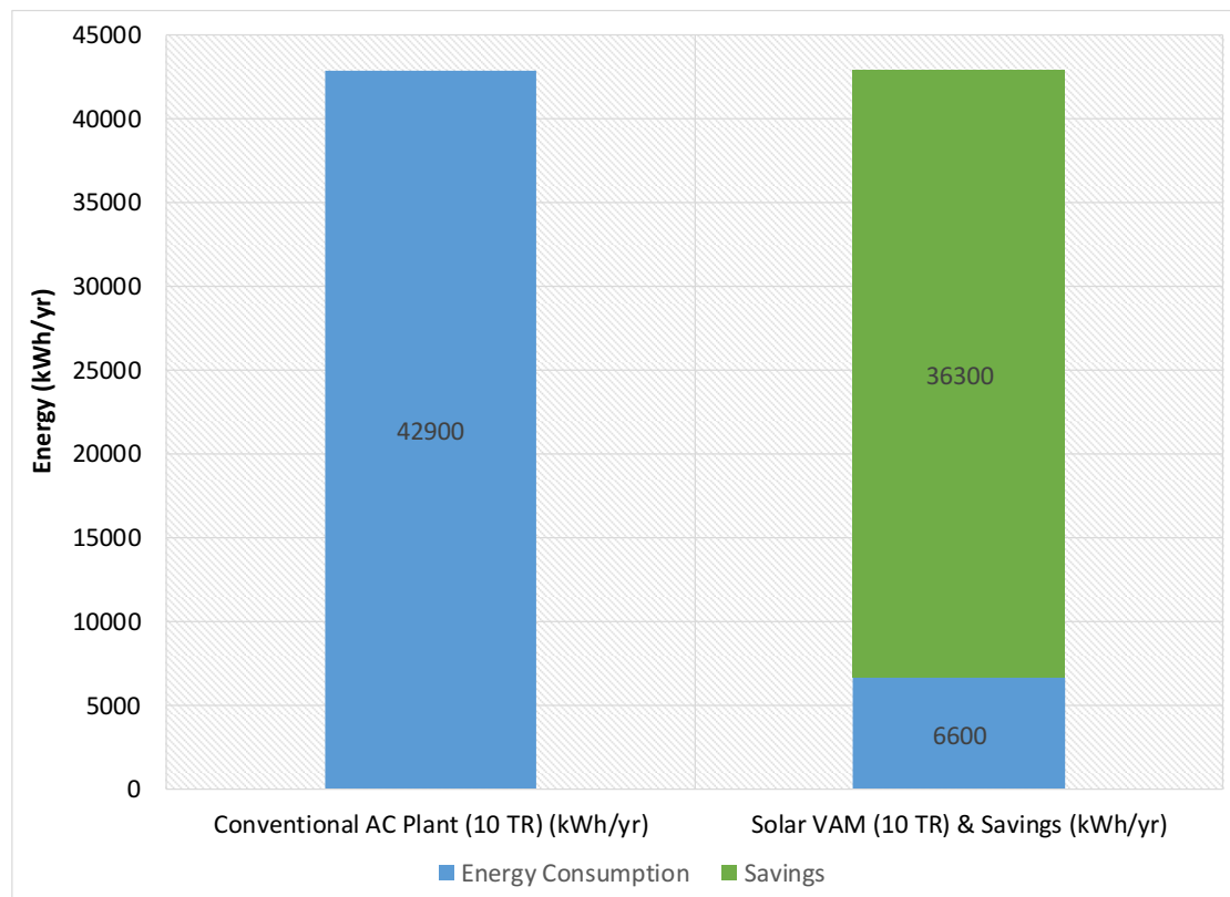
Figure 39 | Energy Consumption and Savings – 10 TR System
