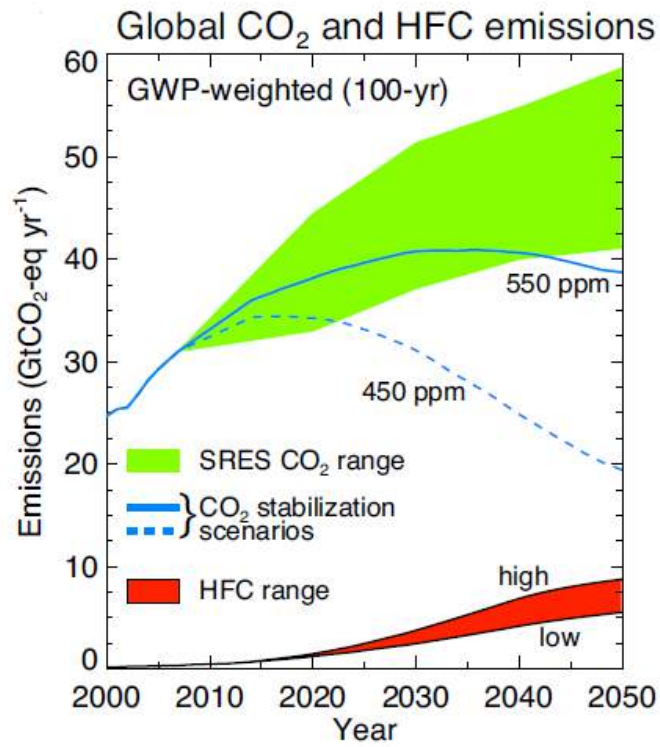
Figure 2 | HFC vs CO 2 Emissions
