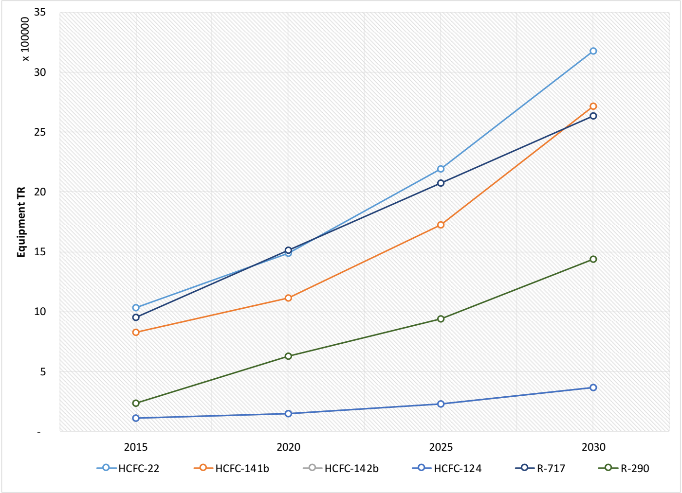
Figure 15 | Industrial Refrigeration Equipment TR Projections (2015-2030)
