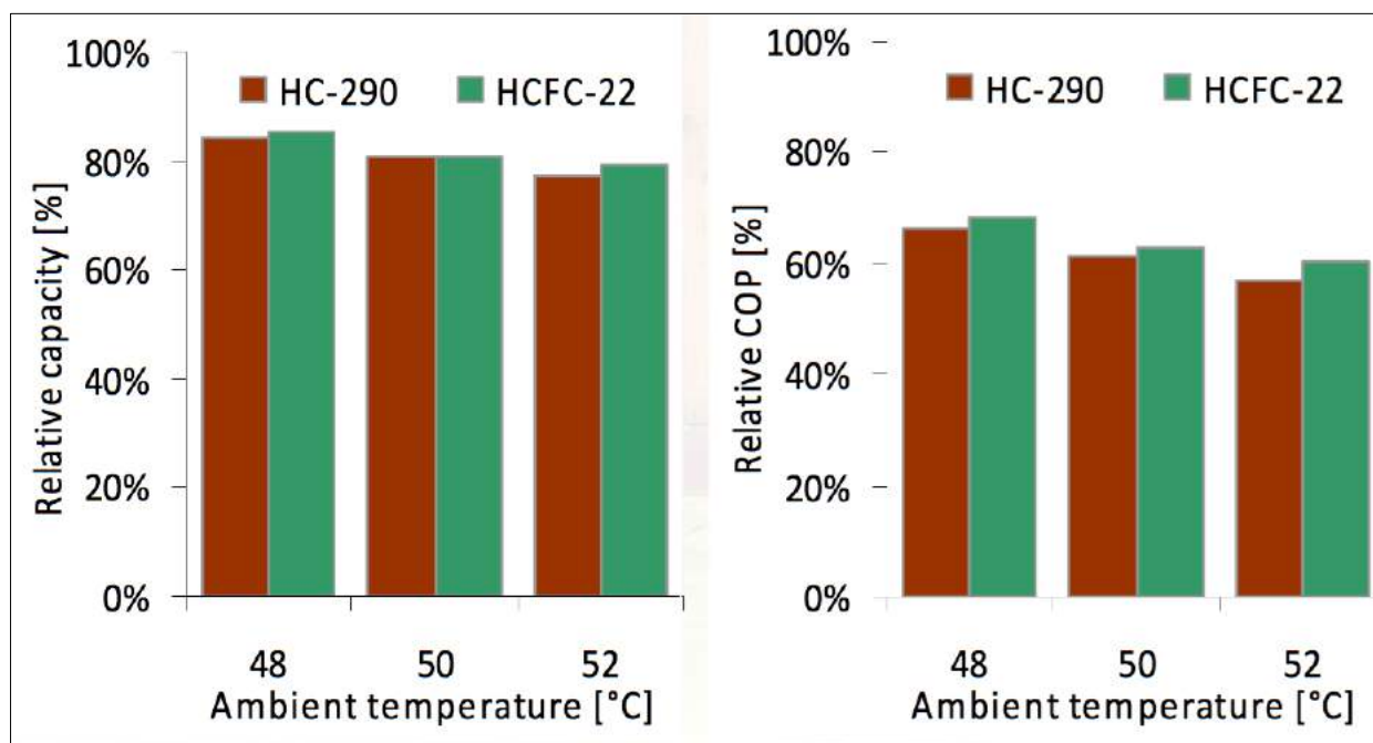
Figure 28 | Comparison of R22 and R290 ACs: I
