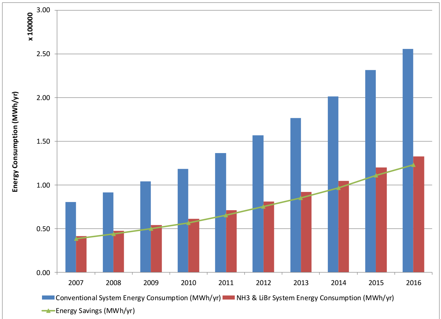
Figure 32 | Energy Consumption: Conventional System vs NH3/LiBr System
