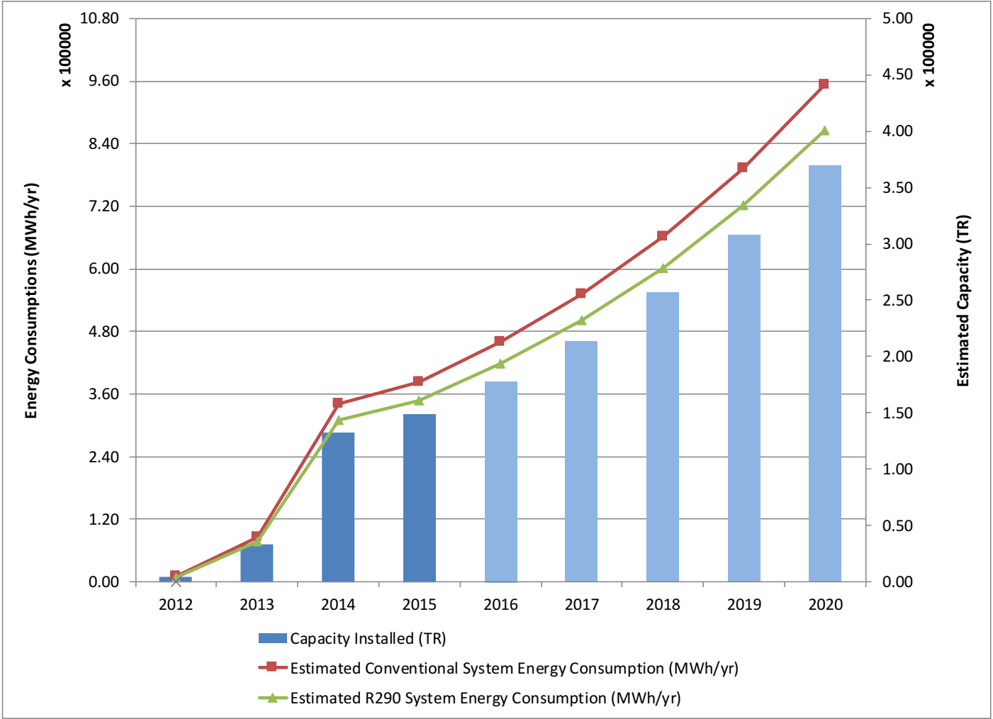
Figure 25 | R290 Growth (TR) & Energy Consumption Projection (MGR Scenario)
