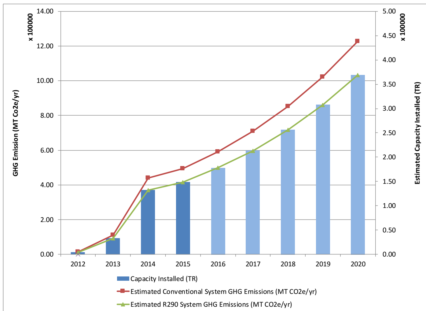
Figure 26 | R290 Growth (TR) & GHG Emission Projection (MGR Scenario)
