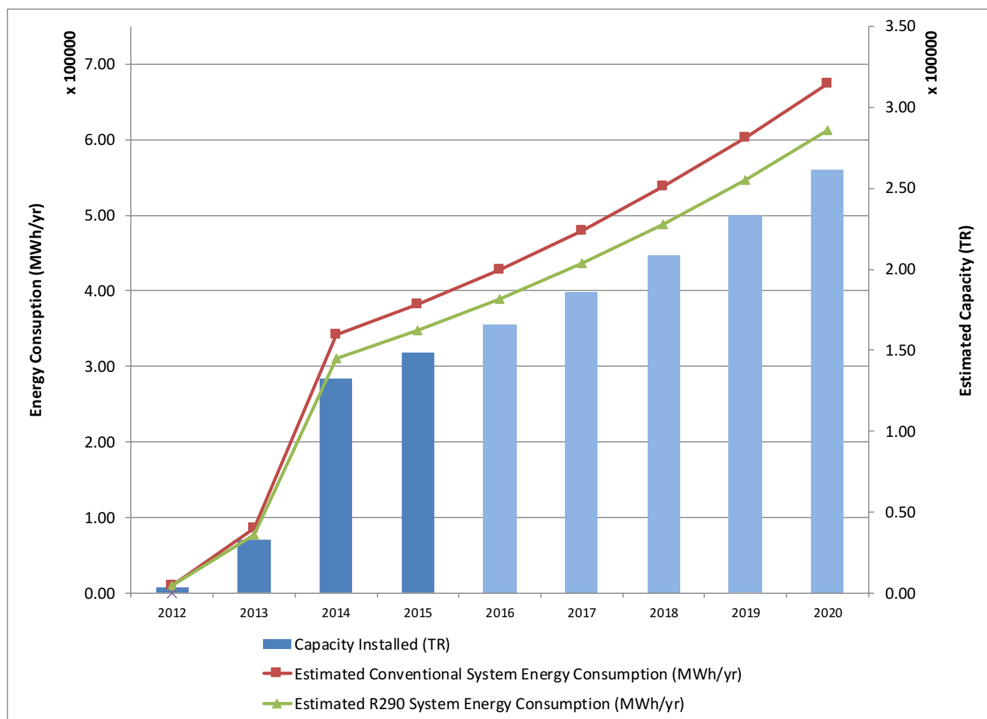
Figure 23 | R290 Growth (TR) & Energy Consumption Projection (BAU Scenario)
