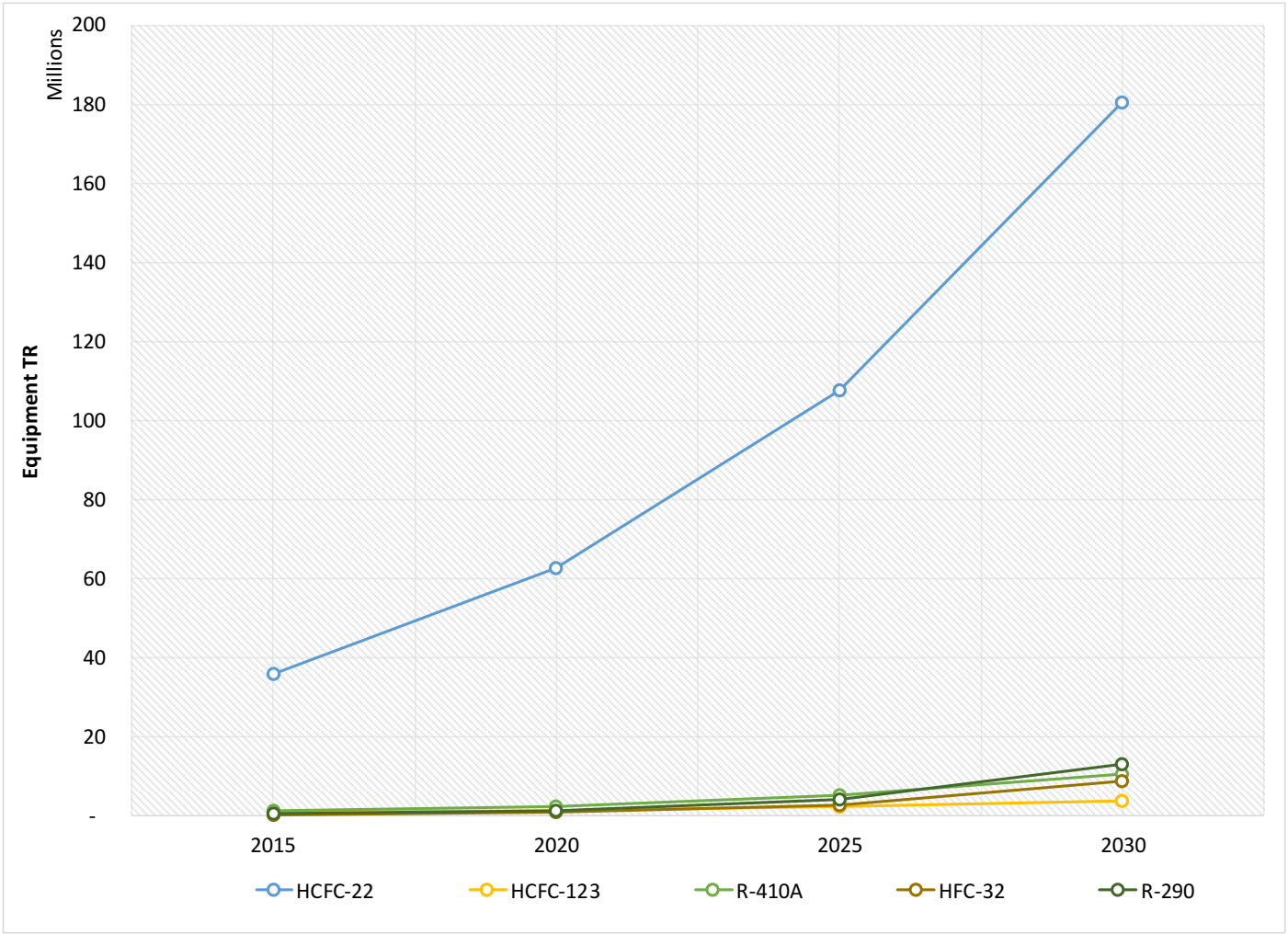
Figure 17 | Residential AC Equipment TR Projections (2015-2030)
