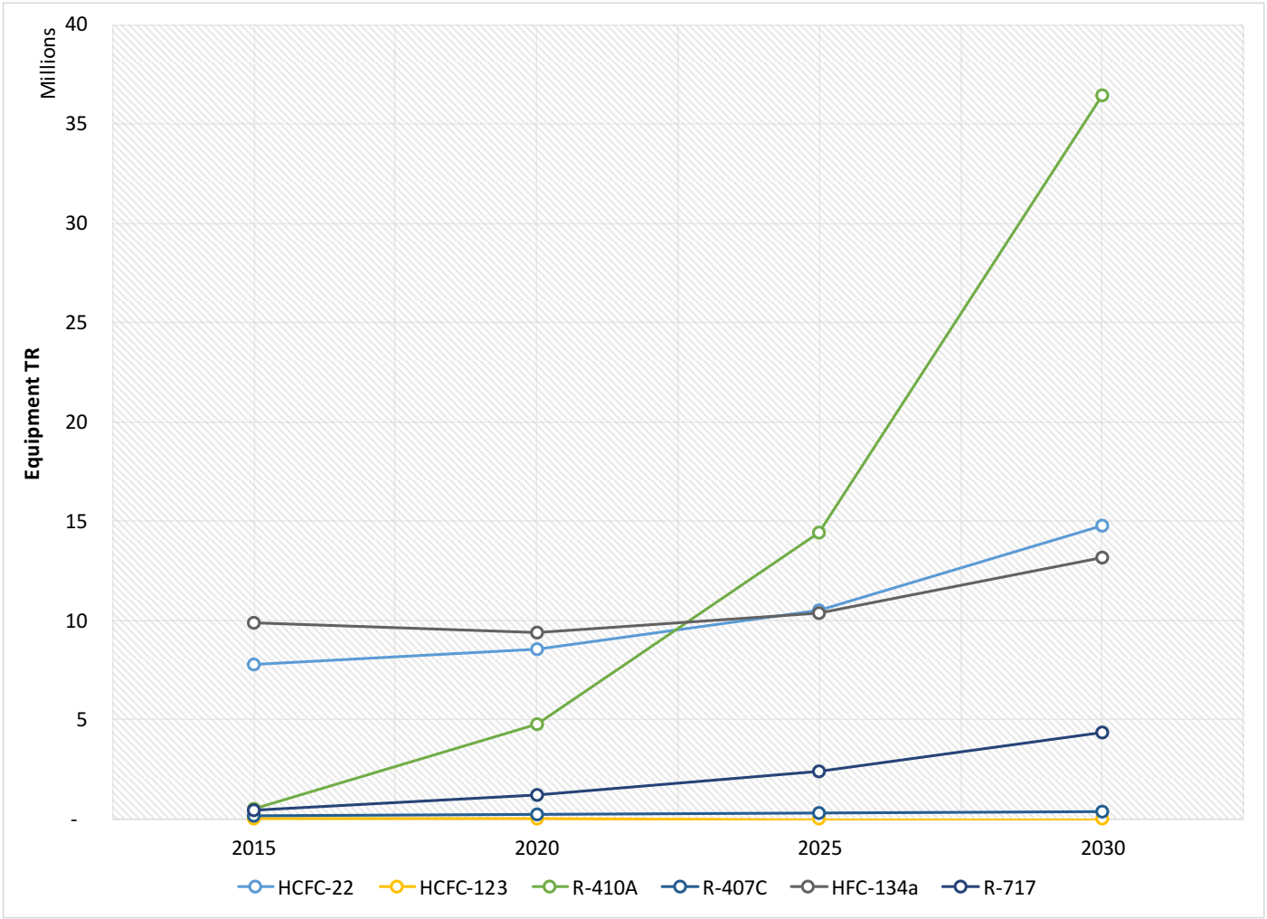
Figure 18 | Commercial AC Equipment TR Projections (2015-2030)
