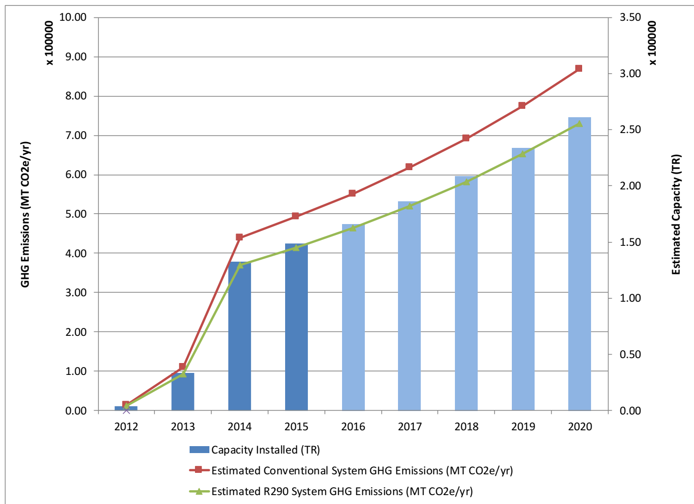
Figure 24 | R290 Growth (TR) & GHG Emission Projection (BAU Scenario)
