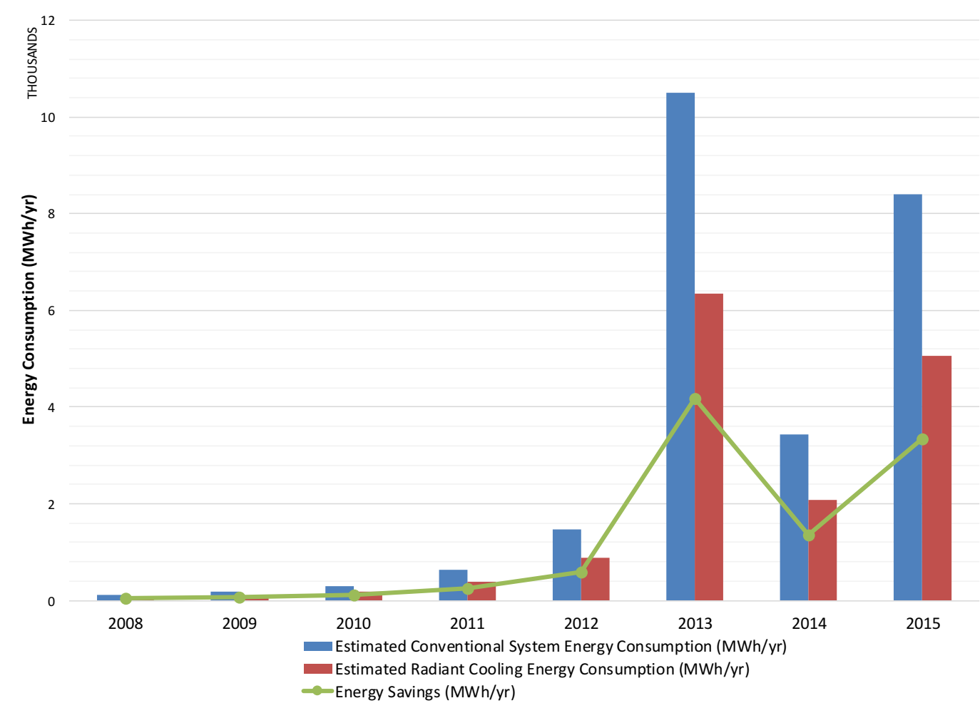
Figure 44 | Energy Consumption: Conventional System vs Radiant Cooling
