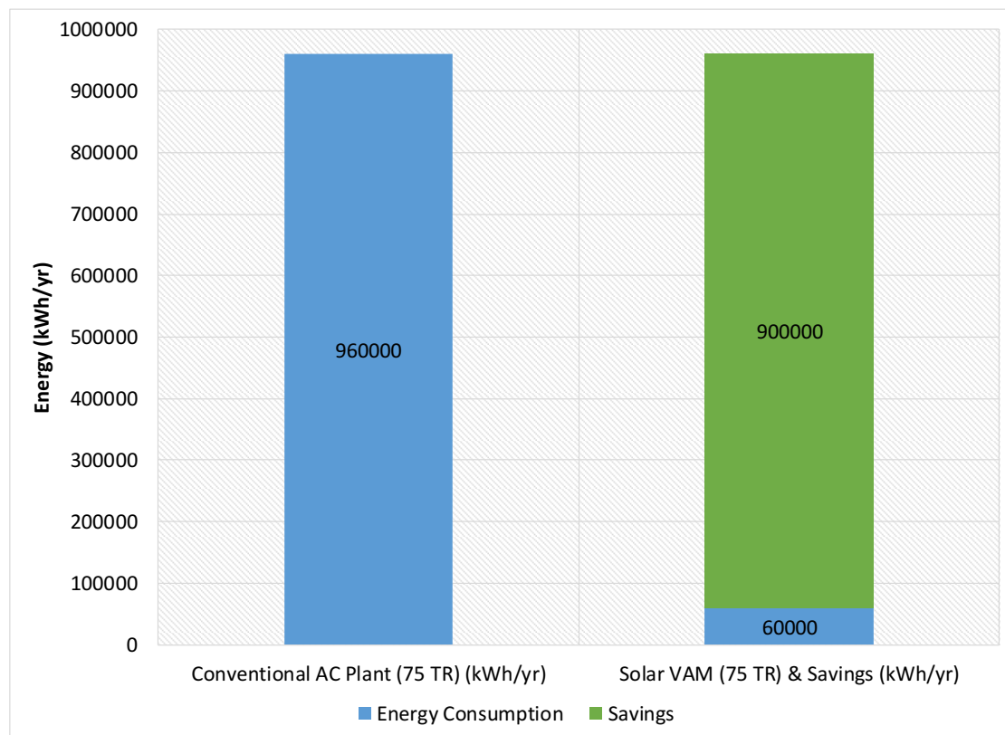
Figure 38 | Energy Consumption and Savings – 75 TR system
