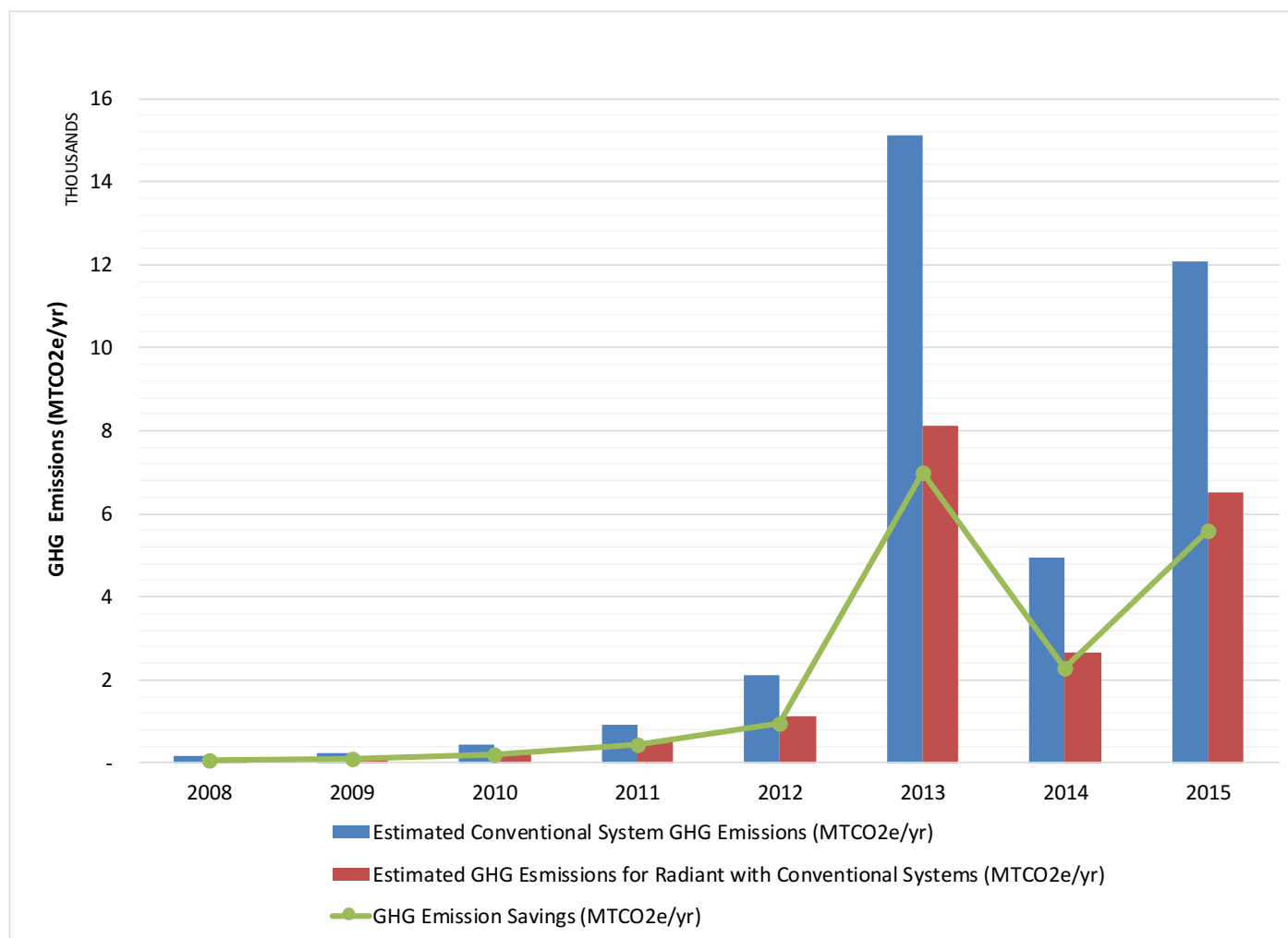
Figure 45 | GHG Emission: Conventional System vs Radiant Cooling
