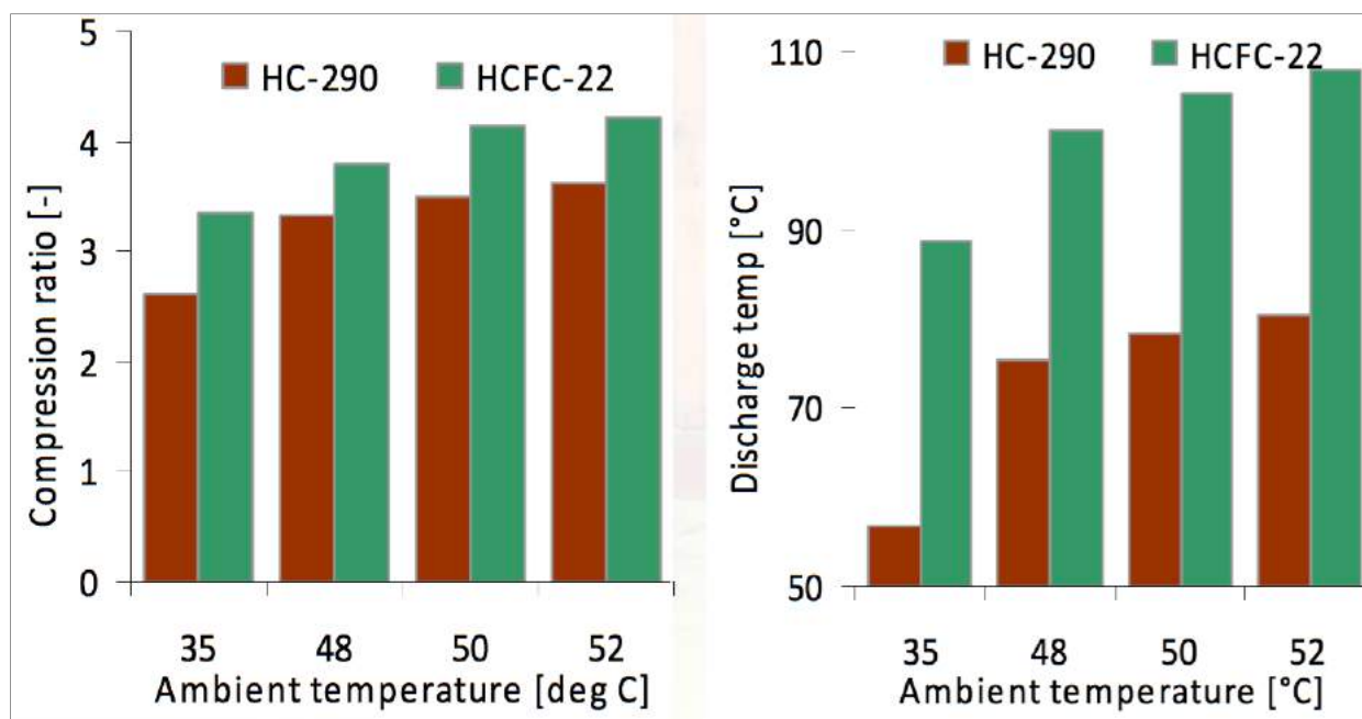
Figure 29 | Comparison of R22 and R290 ACs: II
