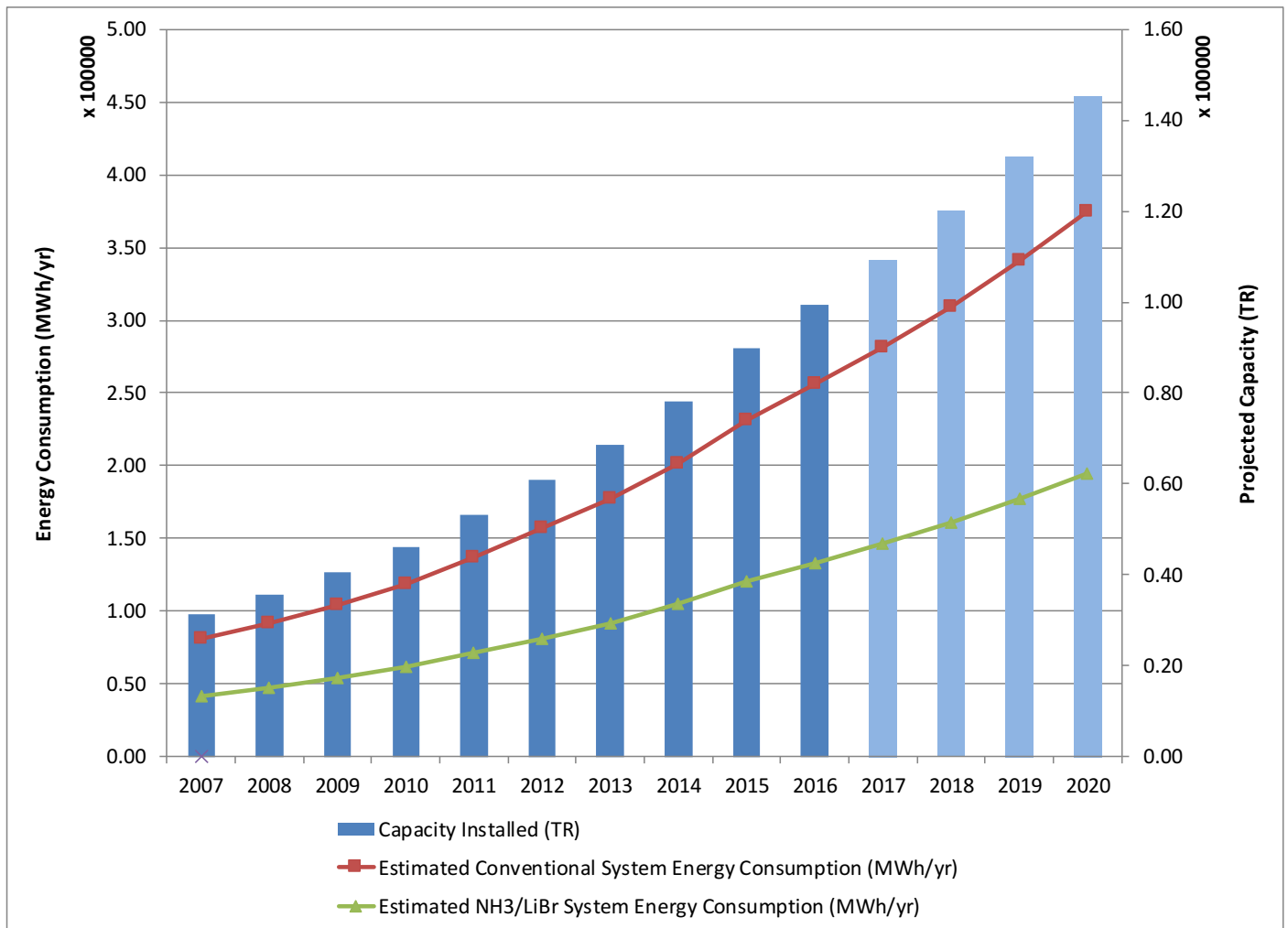
Figure 36 | NH3/LiBr VAM Growth (TR) & Energy Consump. Projection (MGR Scenario)
