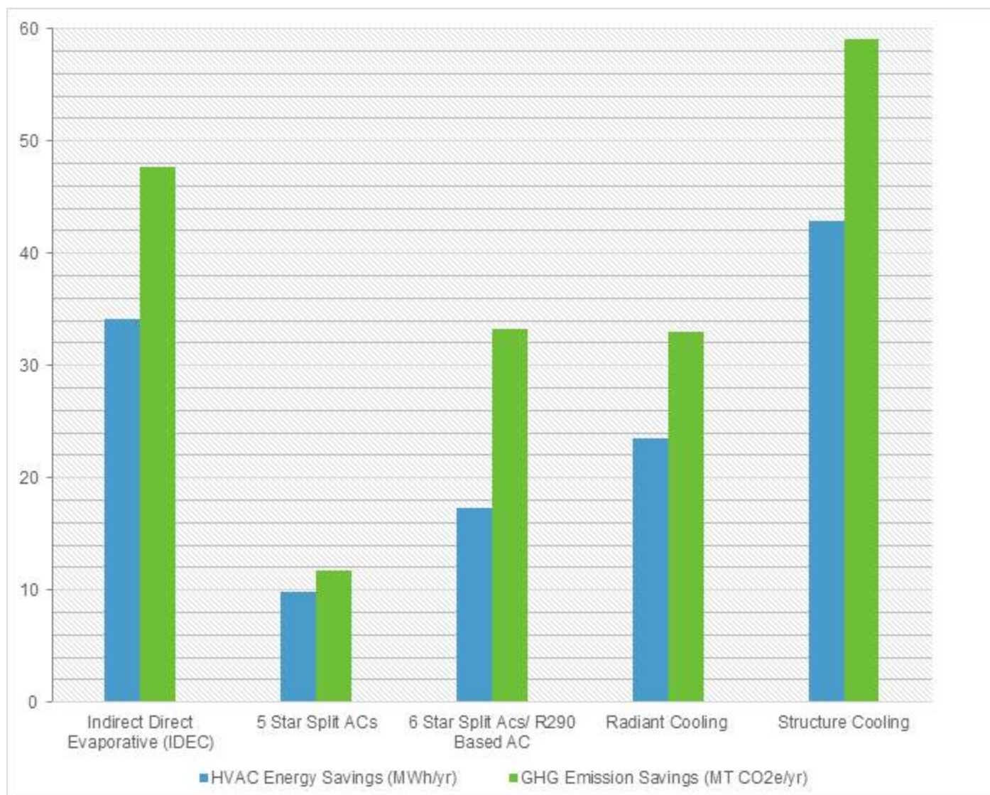
Figure 59 | Energy & GHG Savings – Natural Refrigerant based technologies
