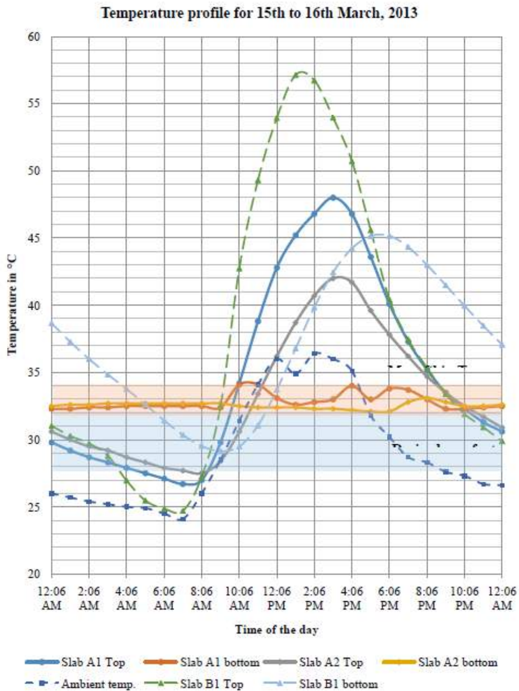
Figure 48 | Structure Cooling Case Study: Temperature Profile
