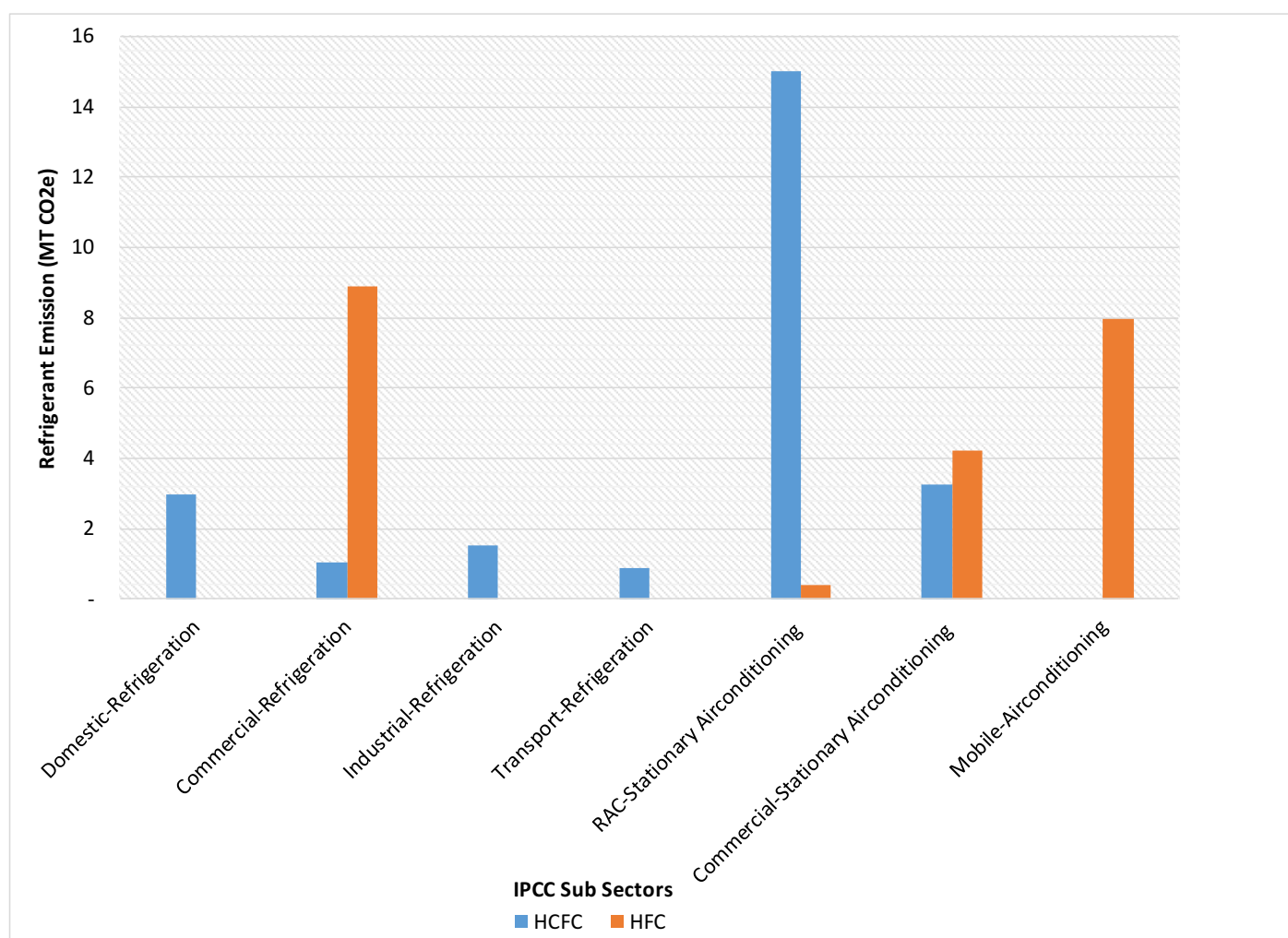
Figure 8 | Refrigerant Emissions- Conservative Scenario (2015)
