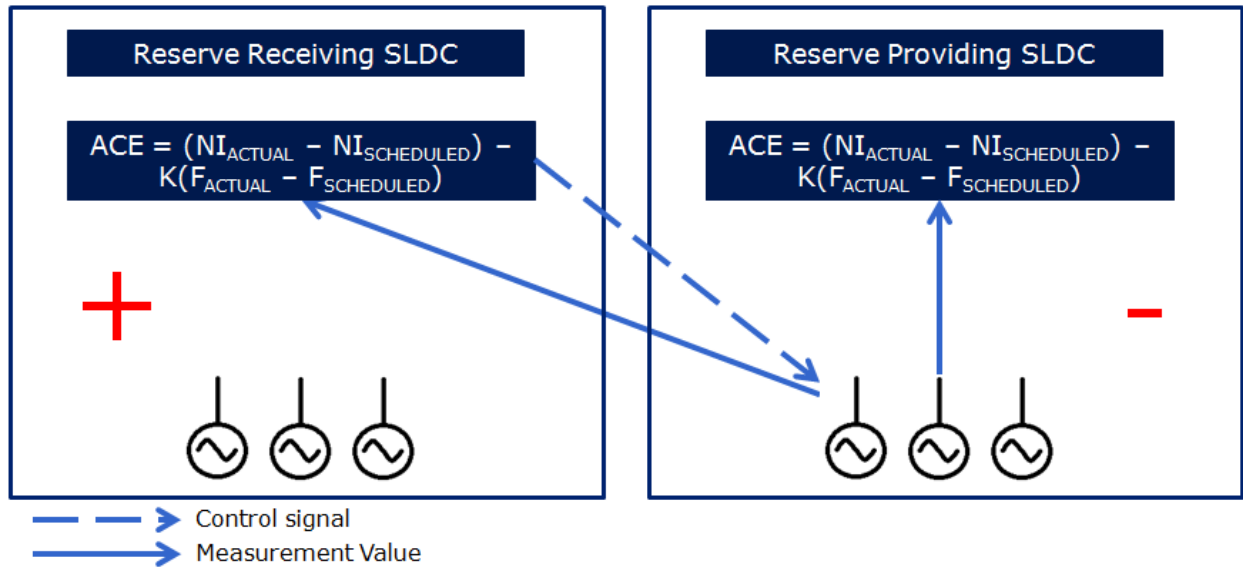
Figure 17: Designated Resources with Pluralistic Control : Secondary Control - Alternative 1
