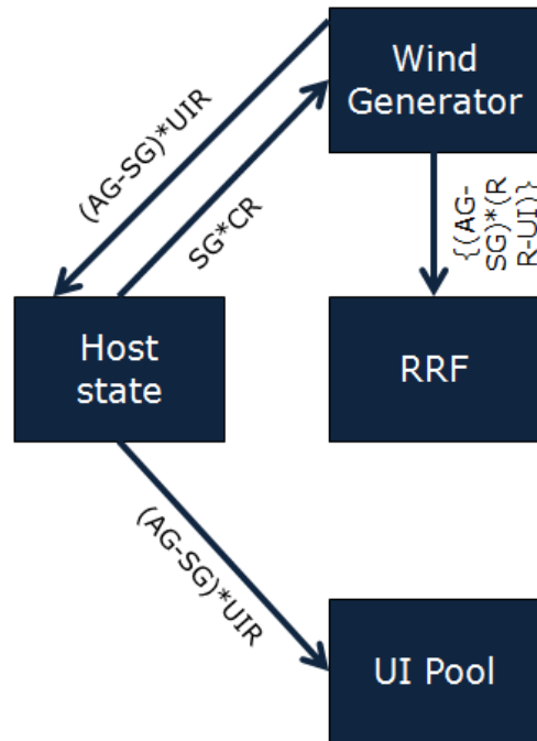
Figure 36: Deviation from Scheduled Generation within -30%
