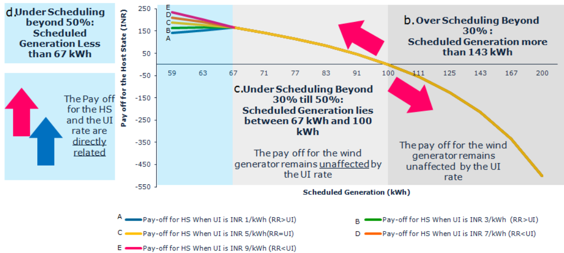
Figure 10: Pay-off for the Host State under the current RRF mechanism
