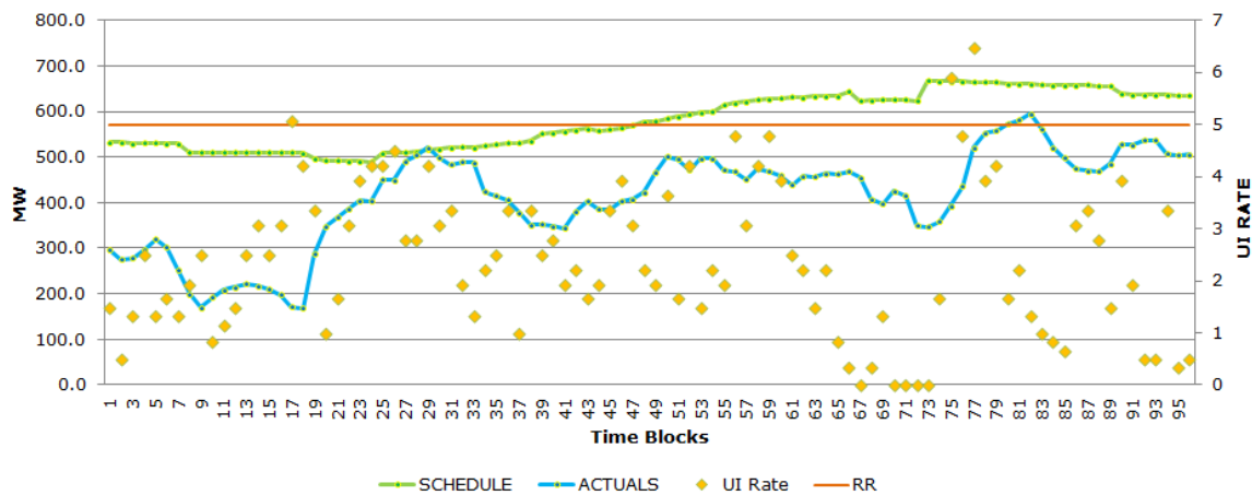
Figure 15: Trend line showing the difference between the SG and AG in Tamil Nadu on 15th July 2013
