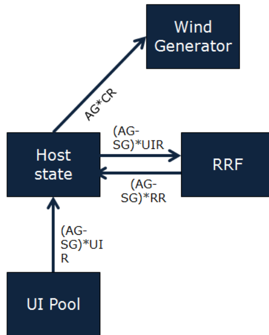
Figure 25: Deviation from Scheduled Generation within +30%
