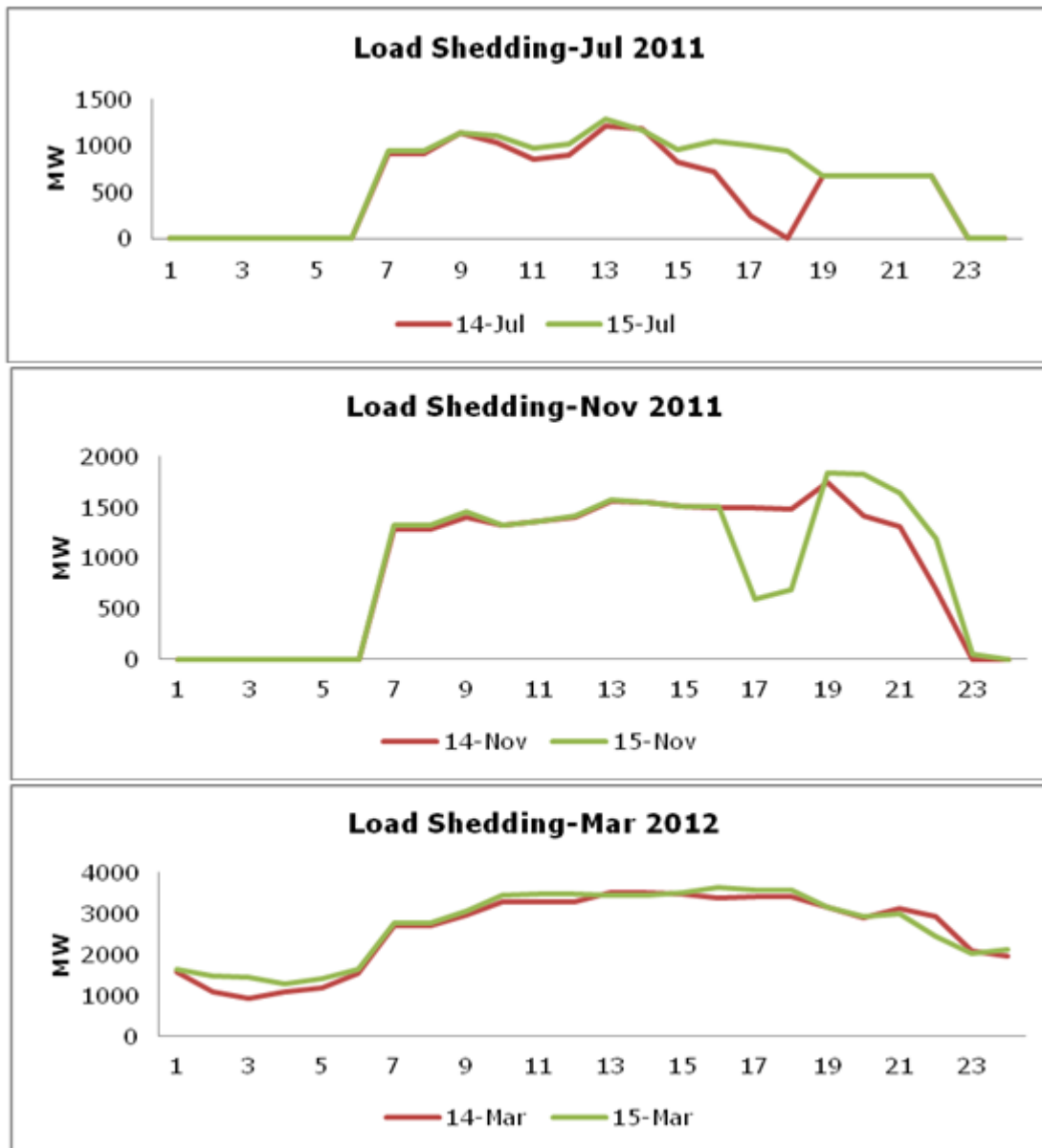
Figure 24: Load shedding in Tamil Nadu
