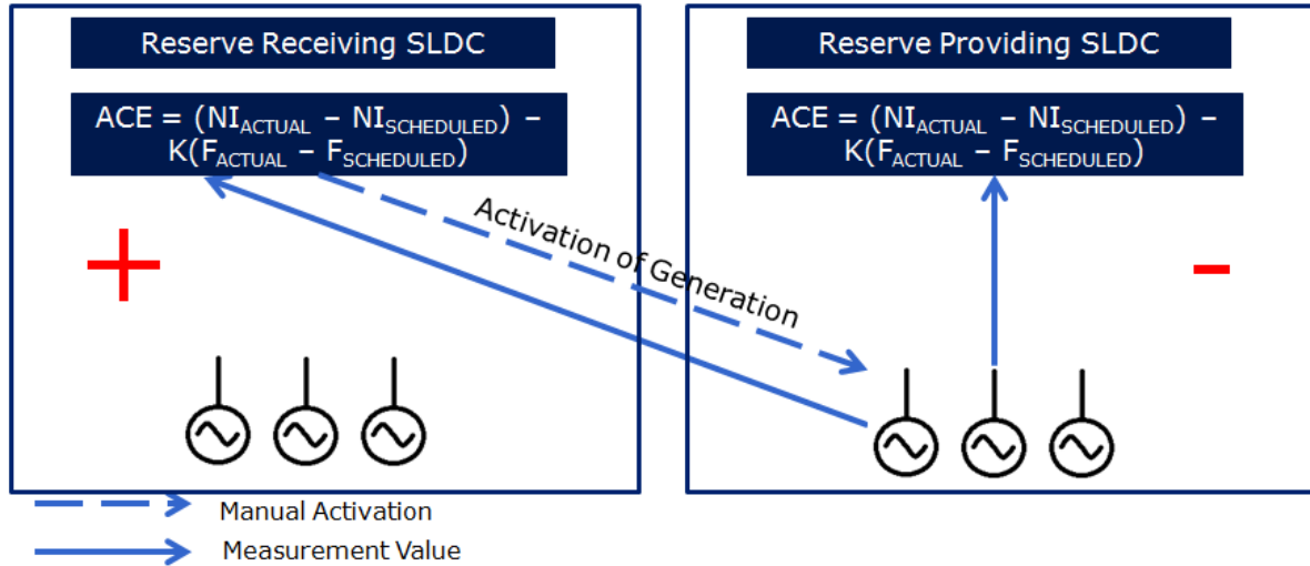
Figure 19: Designated Resources with Pluralistic Control : Tertiary Control - Alternative 1
