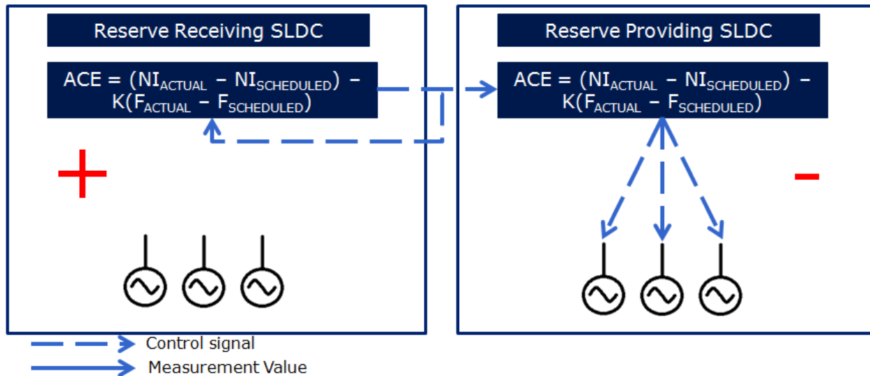
Figure 18: Designated Resources with Pluralistic Control: Secondary Control - Alternative 2
