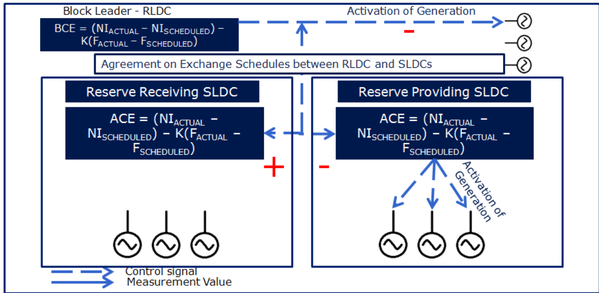
Figure 23: Hierarchical Control with Ancillary Services Market: Tertiary Control
