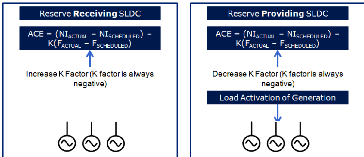
Figure 16: Designated Resources with Pluralistic Control - Primary Control
