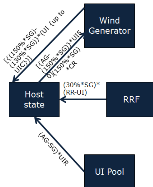
Figure 33: Deviation from Scheduled Generation beyond +50%
