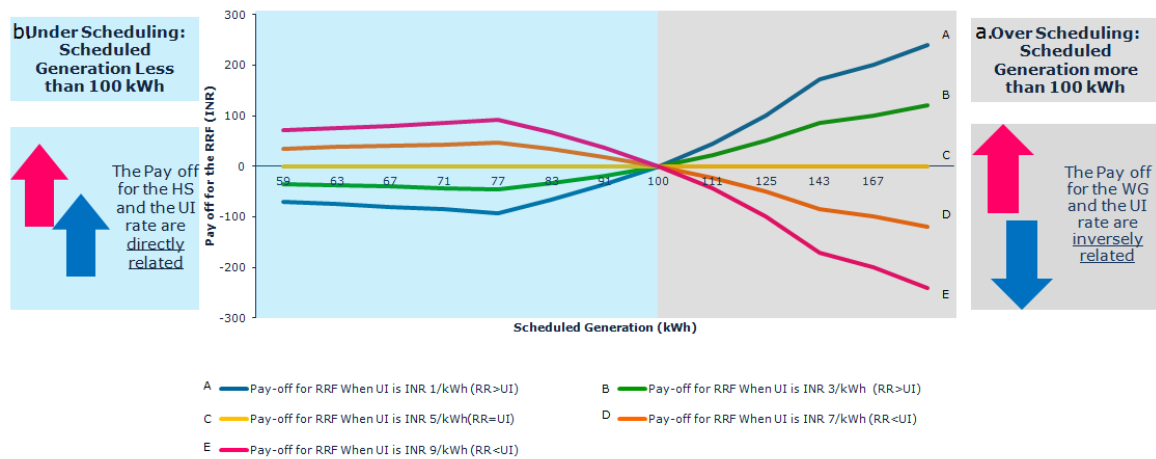
Figure 11: Pay-off for the RRF under the current RRF mechanism
