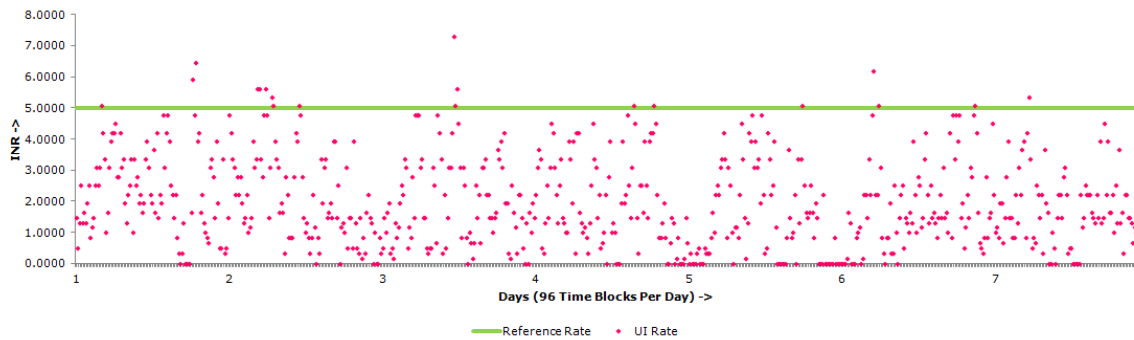
Figure 14: UI Rate and RR rate: Trend over a typical week (96 Time blocks per day) (15/07/2013 to 21/07/2013)
