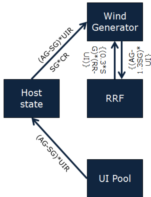
Figure 35: Deviation from Scheduled Generation beyond +30%
