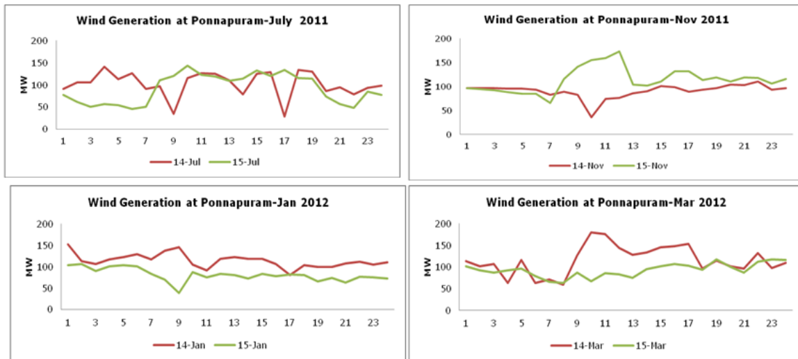
Figure 3: Wind Generation in Tamil Nadu during 2011
