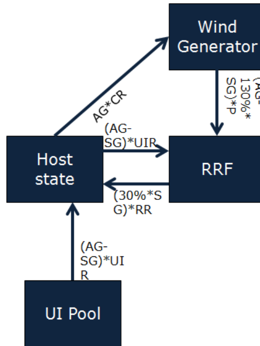
Figure 26: Deviation from Scheduled Generation beyond +30%
