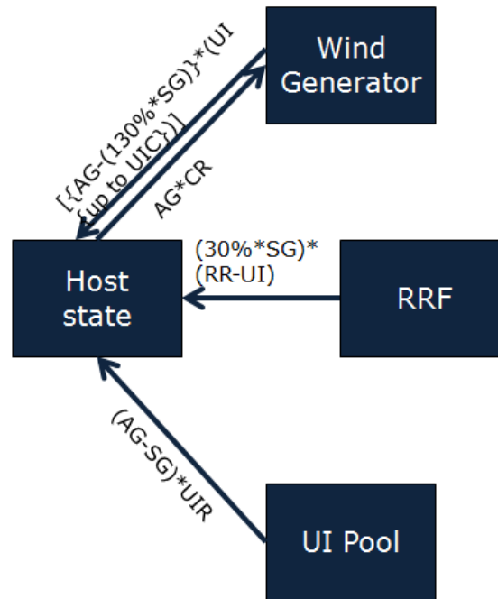
Figure 30: Deviation from Scheduled Generation between +30% and +50%
