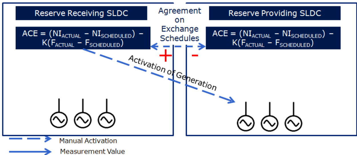
Figure 20: Designated Resources with Pluralistic Control : Tertiary Control - Alternative 2
