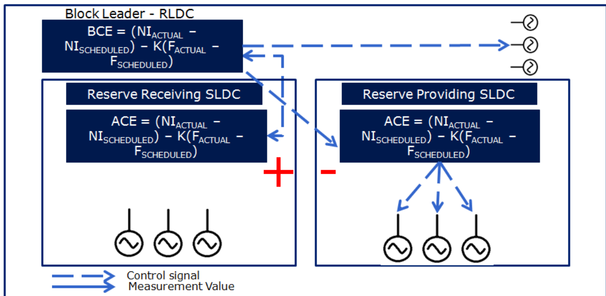
Figure 22: Hierarchical Control with Ancillary Services Market: Secondary Control
