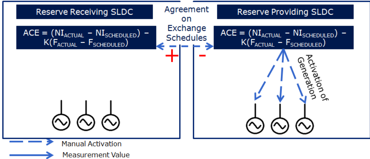
Figure 21: Designated Resources with Pluralistic Control : Tertiary Control - Alternative 3
