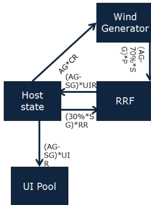
Figure 28: Deviation from Scheduled Generation beyond -30%
