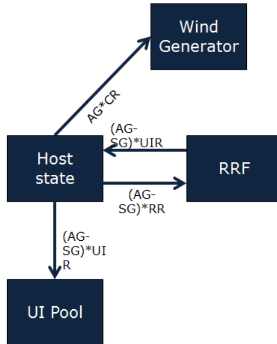
Figure 27: Deviation from Scheduled Generation within -30%
