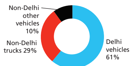
Particulate load
