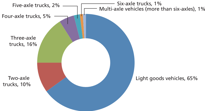
B. Particulate load from different segments of trucks
