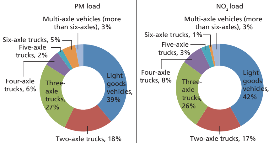
B. Particulate load from different segments of trucks
