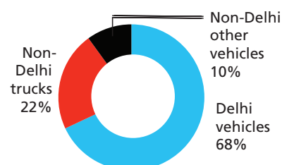
NO x load
